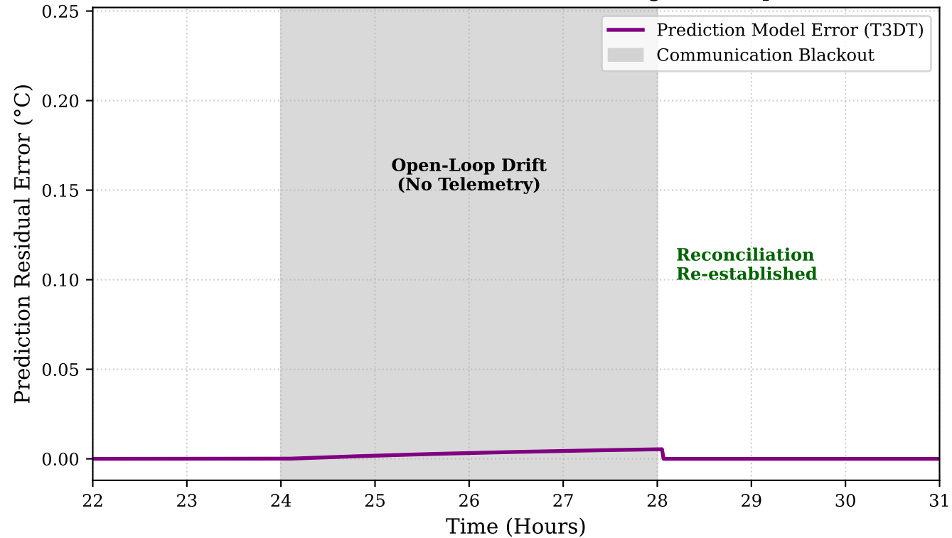
Prediction Error Growth and Convergence (Exp 4)
