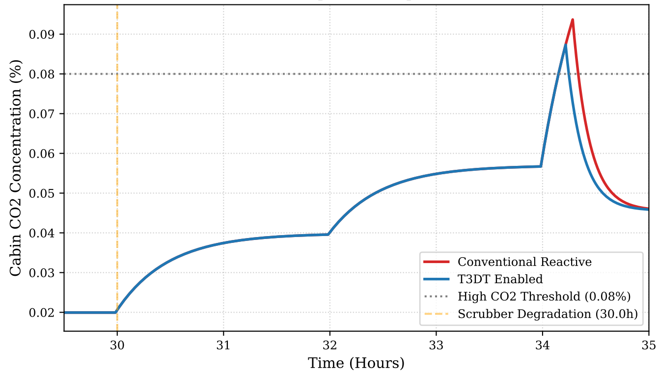
ECLSS Scrubber Response Comparison: Scenario C
