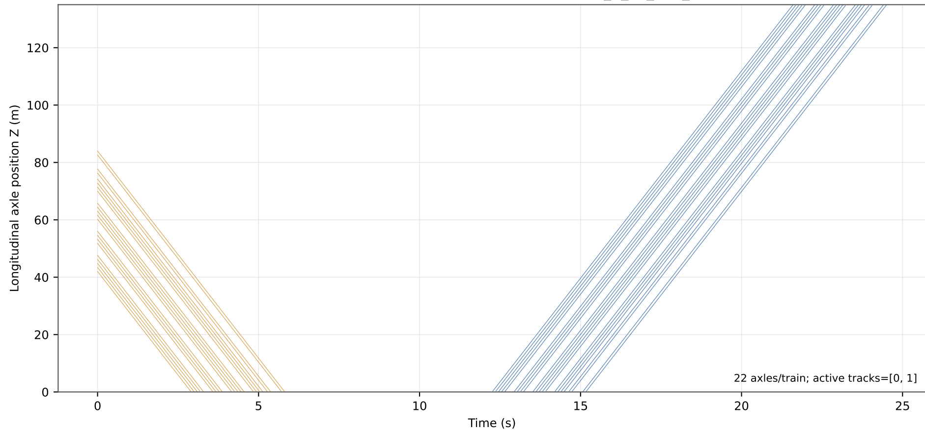
Causal axle trajectories on active rails — V52_C_E8_C12_2T
