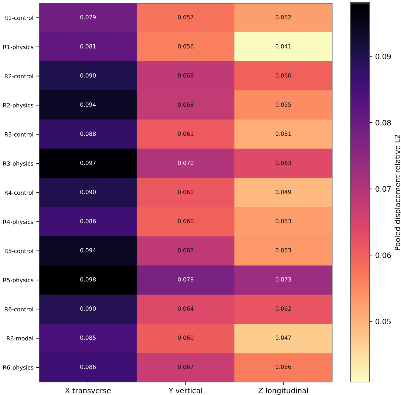
Factorial-panel median error across two seeds
