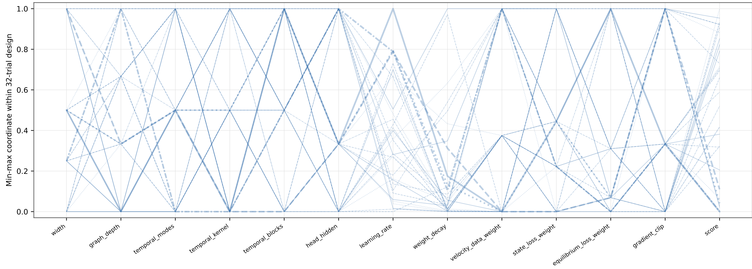
S9 hyperparameter parallel coordinates; thick lines reached high fidelity
