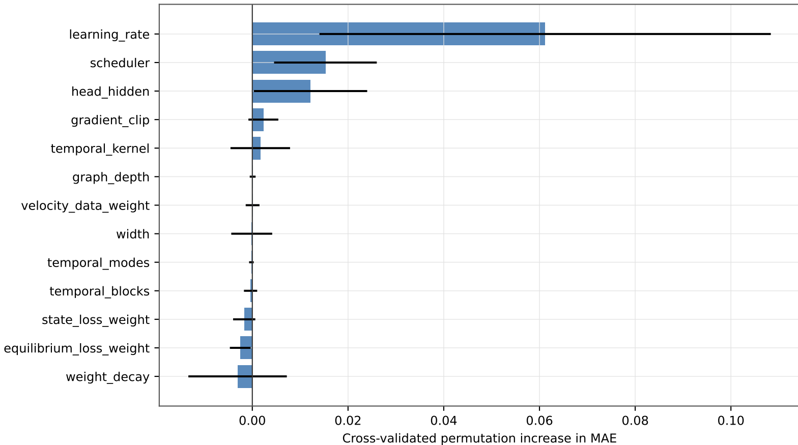
Exploratory S9 hyperparameter importance (n=32)
