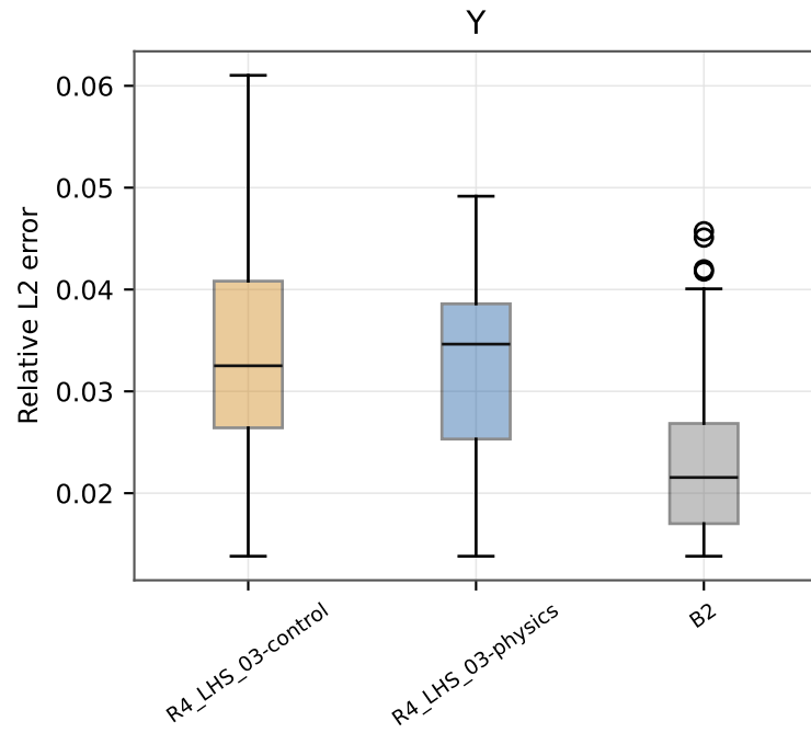
OOF error distributions by model and global component
