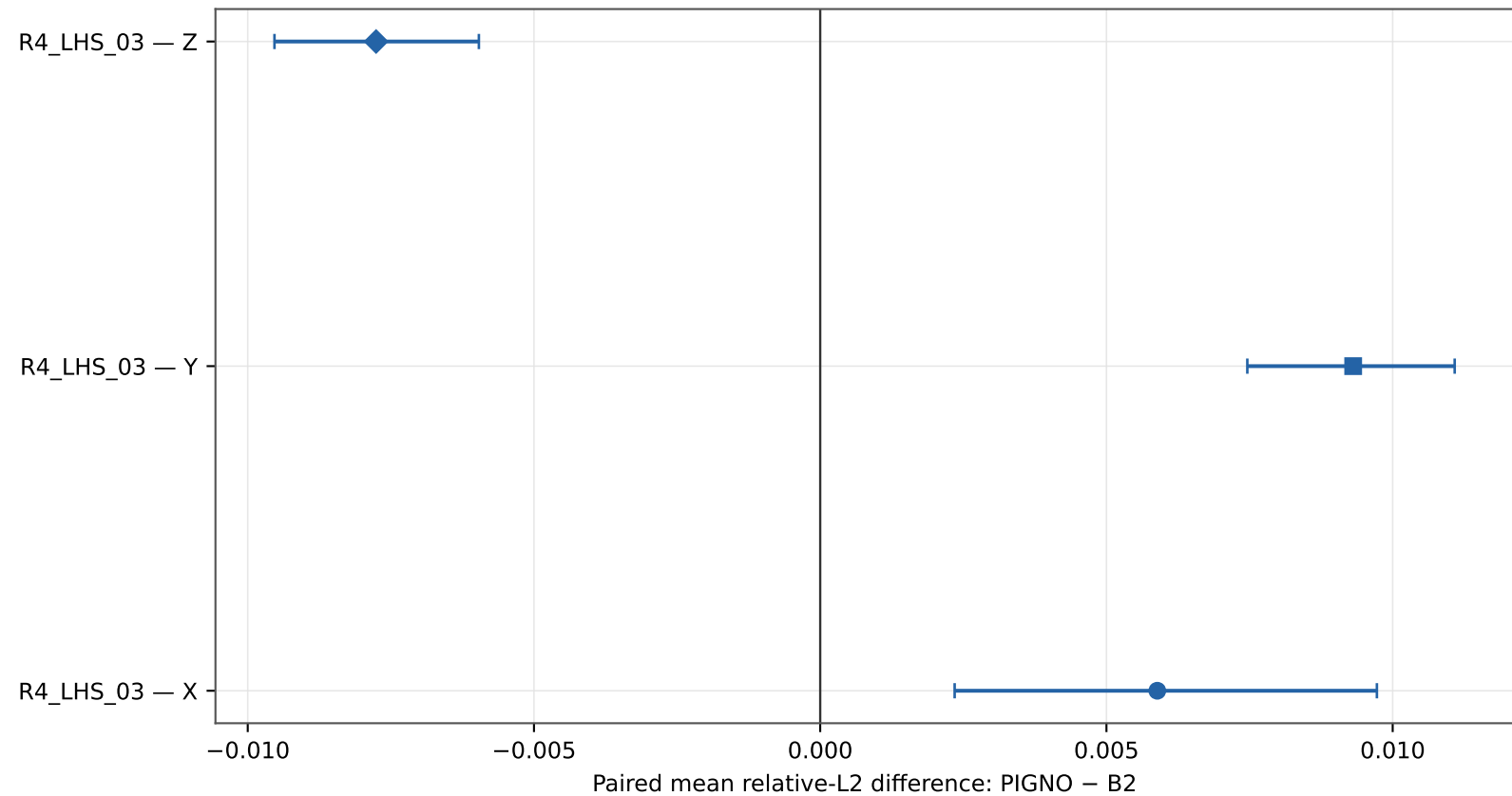
Trajectory-paired OOF improvement versus common B2
