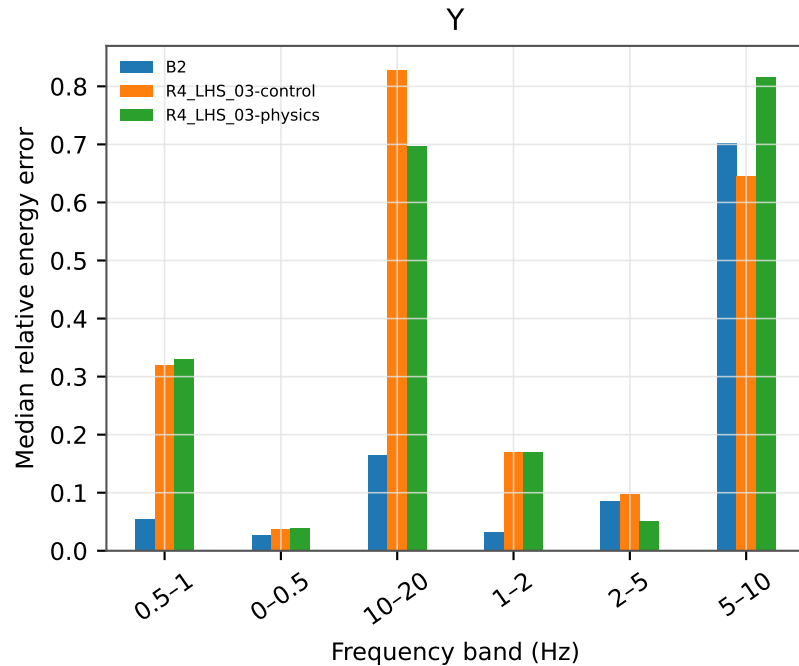
OOF spectral-energy error by frequency band
