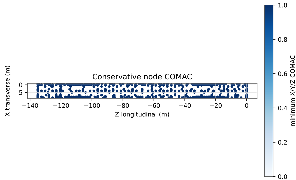
Structural COMAC over the 512 bridge observations
