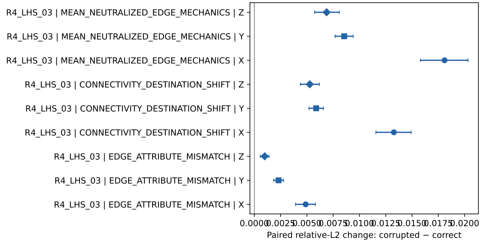
OOF graph-corruption effect
