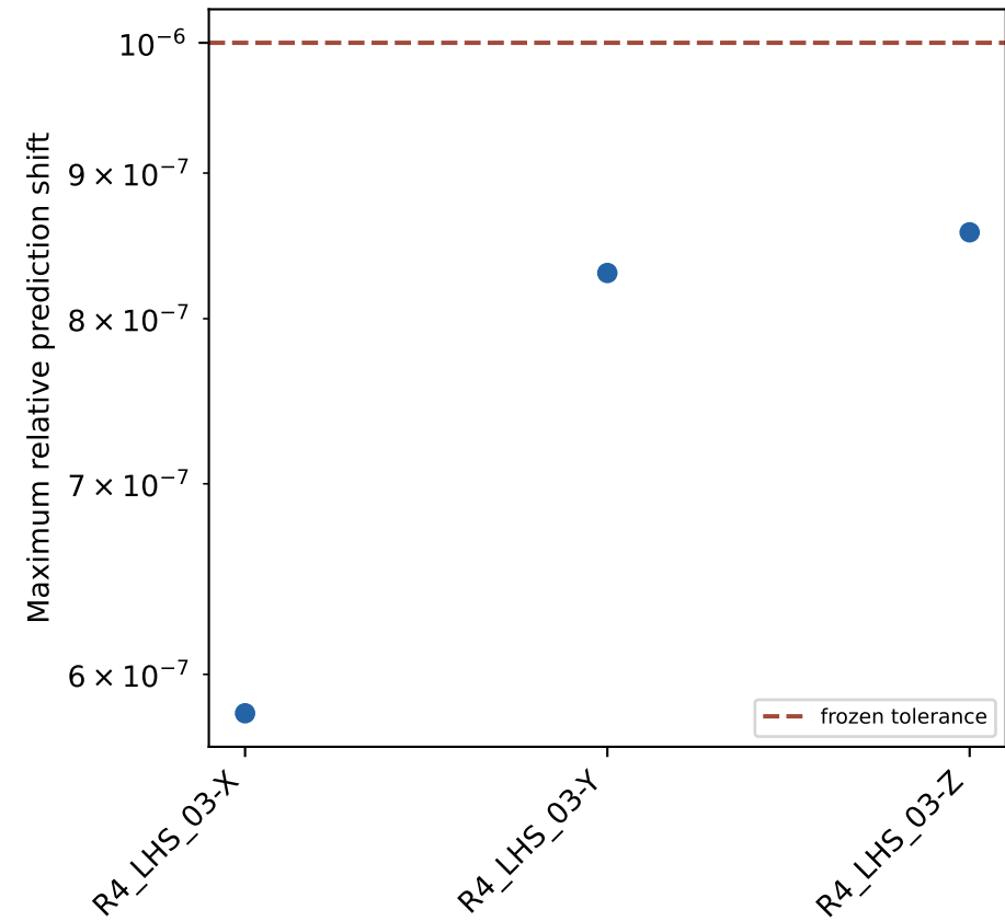
Consistent node-relabel invariance
