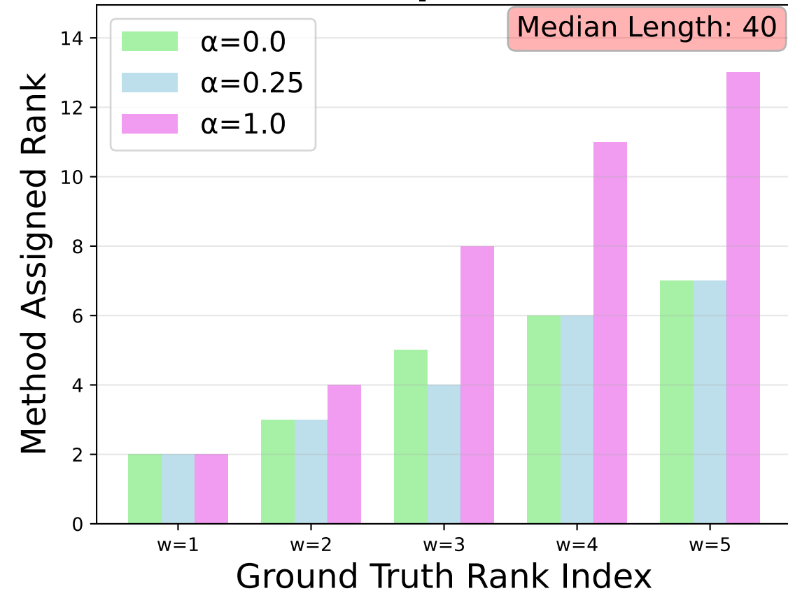
HotpotQA
