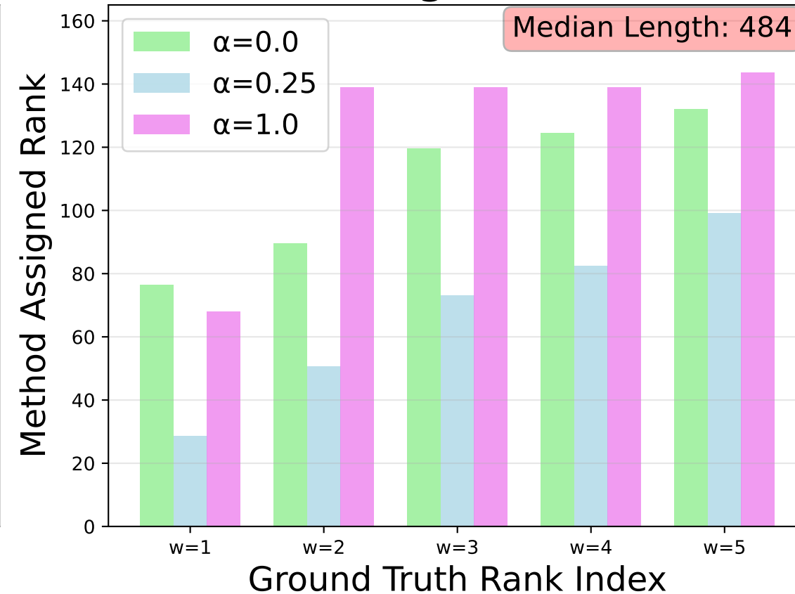
Longbench
