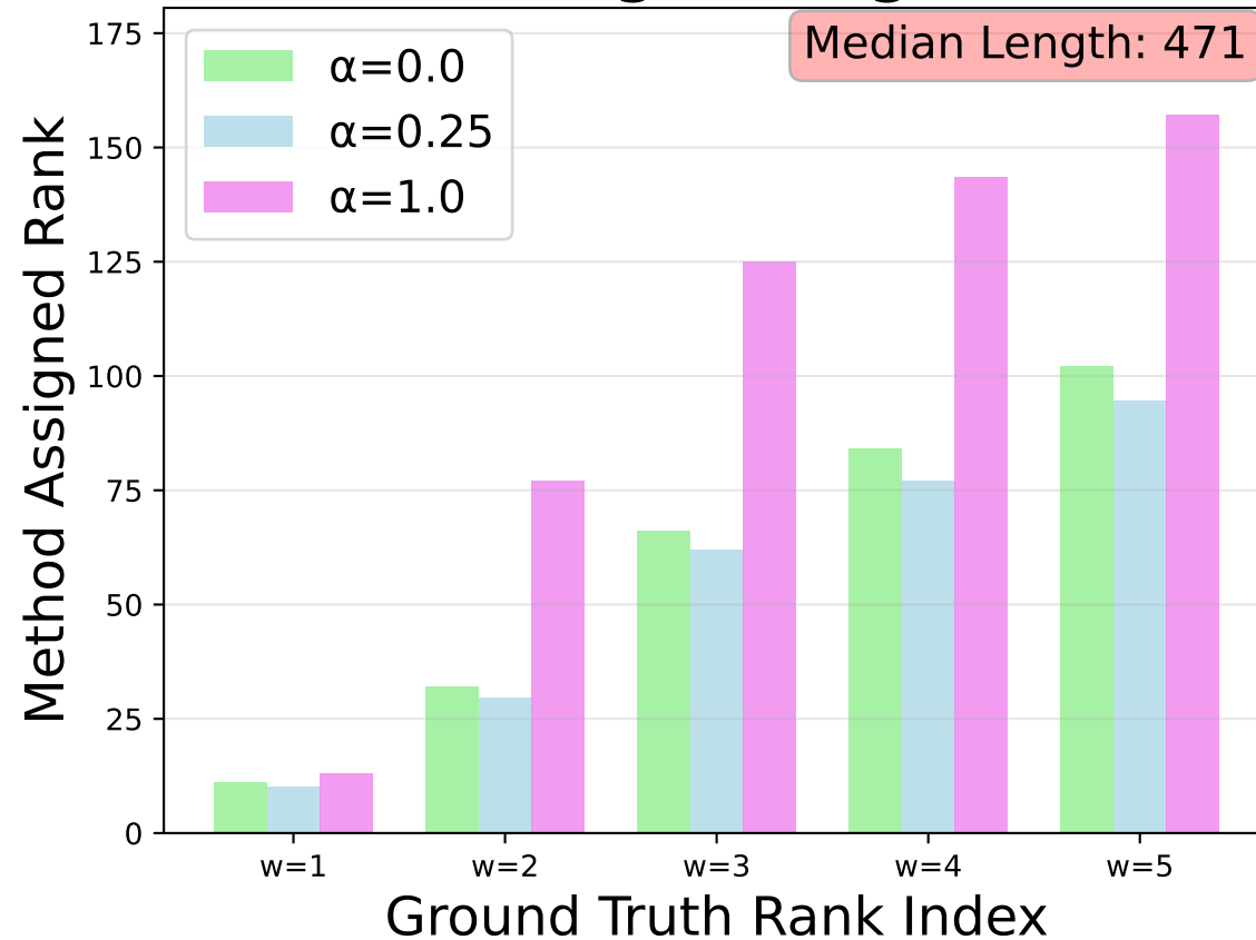
Loogle (long)
