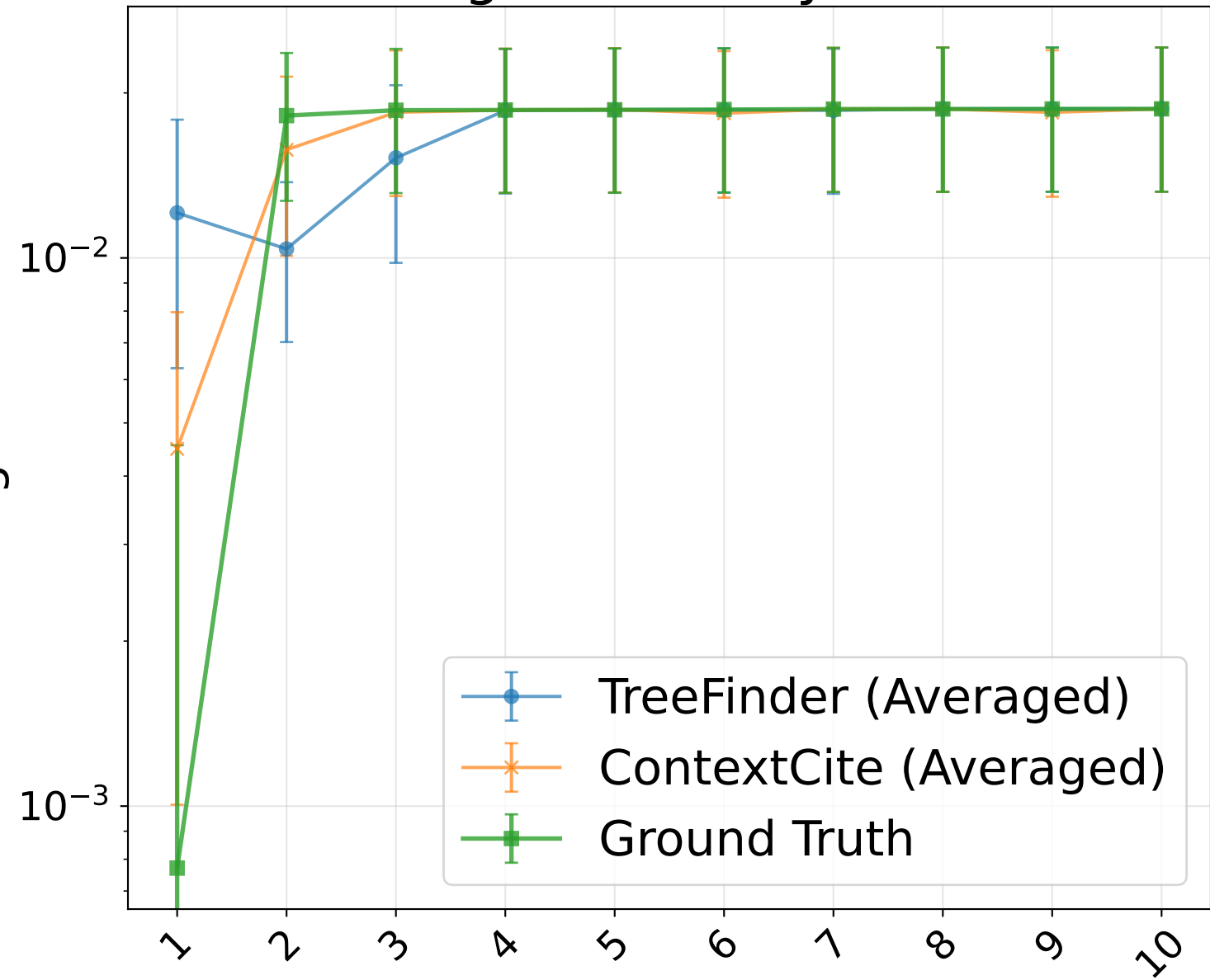
Average Necessity Scores
