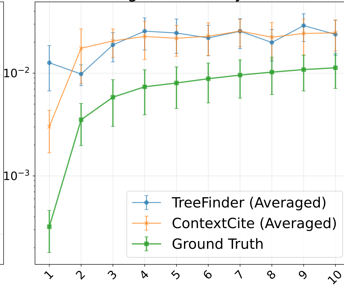
Average Sufficiency Scores
