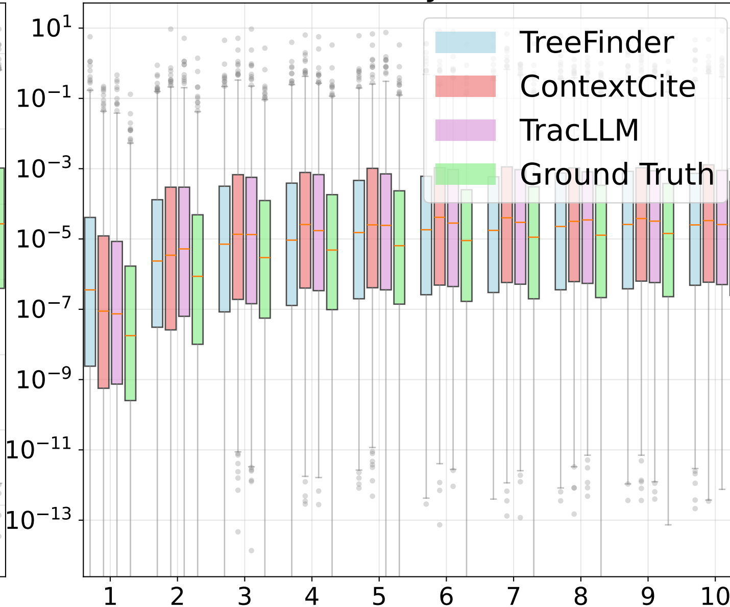
Sufficiency Scores
