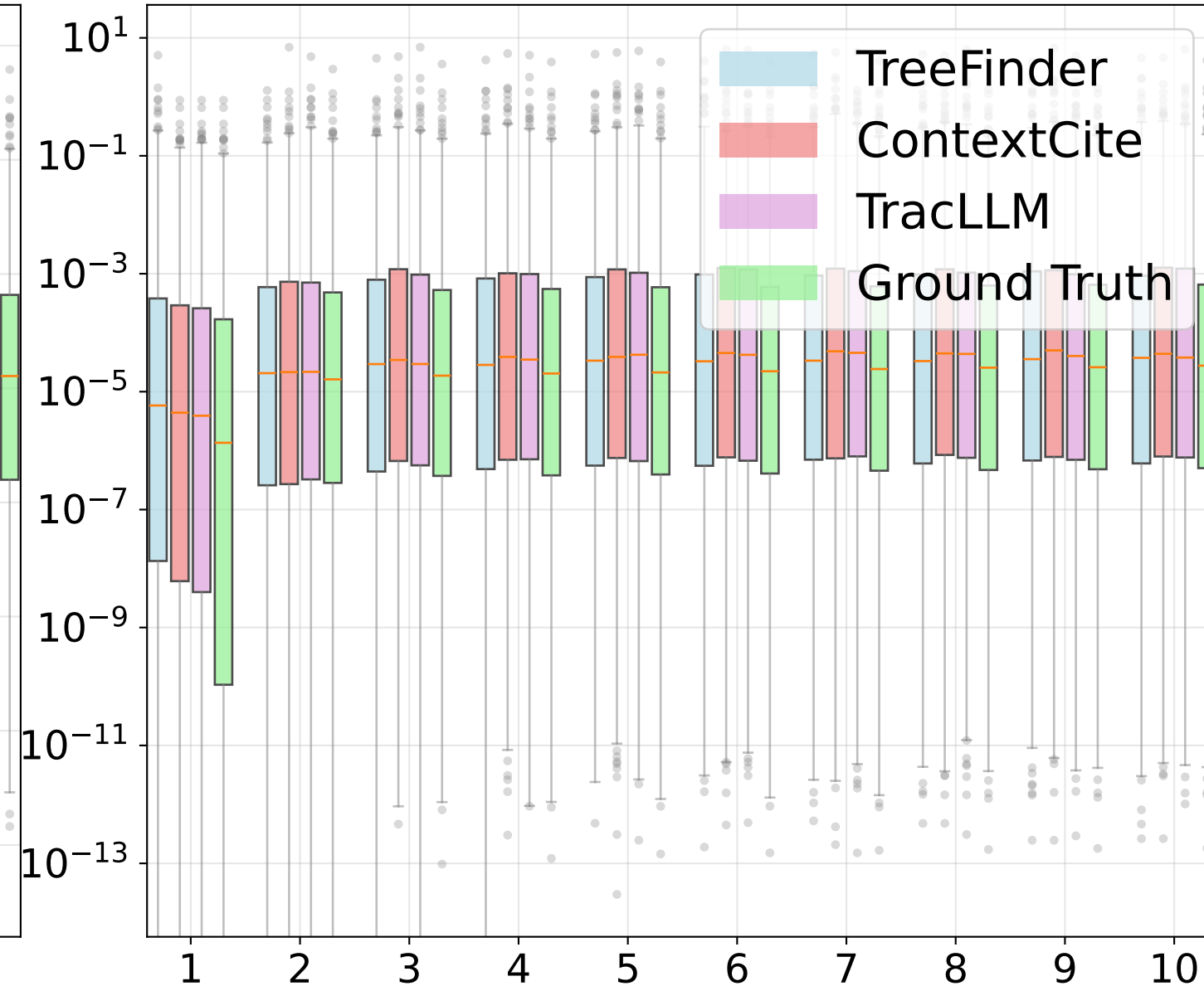
Combined Scores
