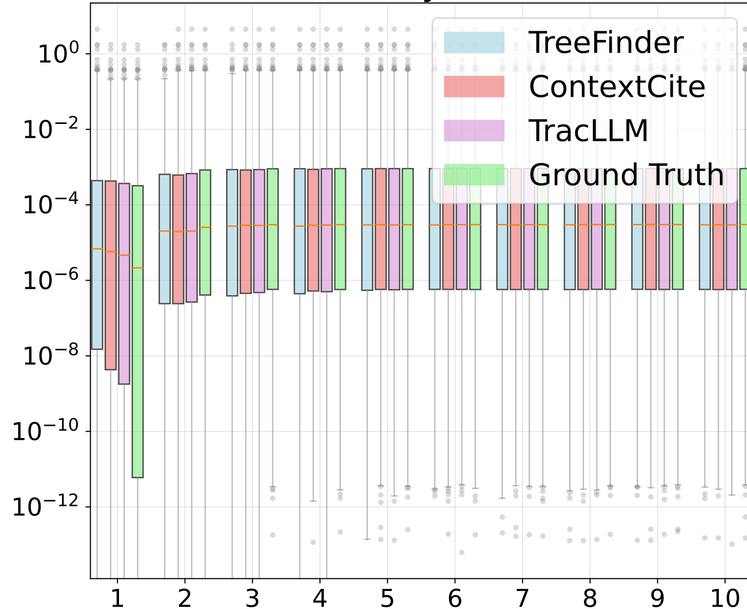
Necessity Scores
