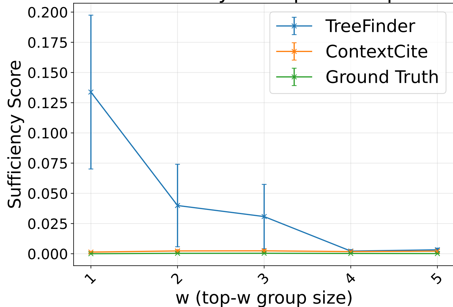
Sufficiency for Top-w Groups
