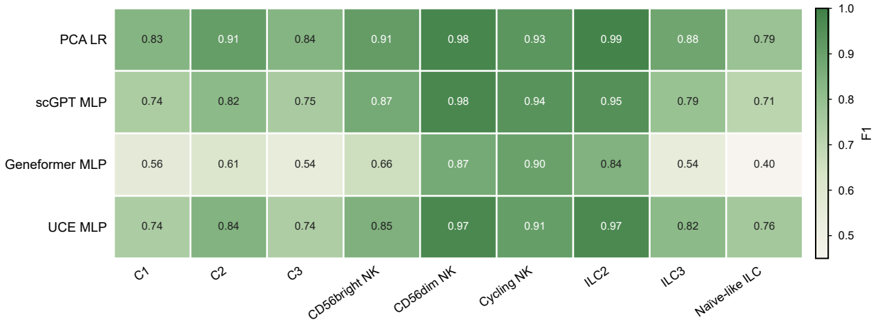
Per-class F1 across selected celltype_l4 models
