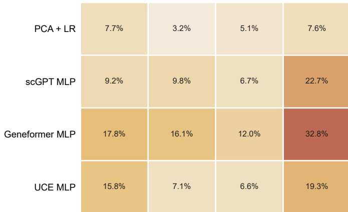
Selected confusion rates
