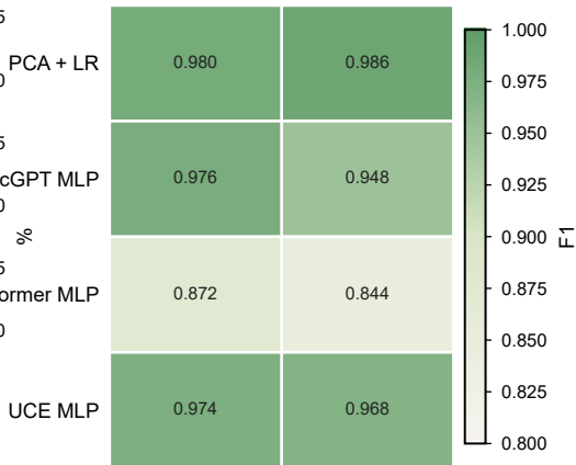
Selected strong classes
