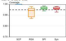
MEPS 40-60, \alpha=0.05
