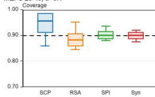
MEPS 20-40, \alpha=0.1
