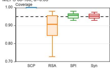
MEPS 60-100, \alpha=0.05
