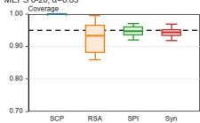
MEPS 0-20, \alpha=0.05
