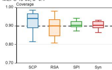
MEPS 40-60, \alpha=0.1
