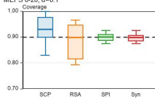
MEPS 0-20, \alpha=0.1
