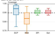
MEPS 60-100, \alpha=0.1
