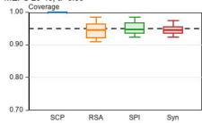
MEPS 20-40, \alpha=0.05
