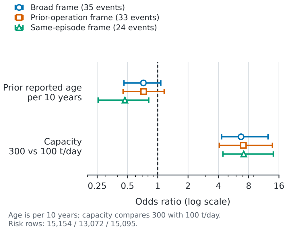
Figure 2: Five-parameter Firth estimates for first reported installed-capacity entry. Capacity is shown as the 300-versus-100 t/day contrast and age per ten years; intervals come from 1,999 whole-lineage bootstrap replications.
