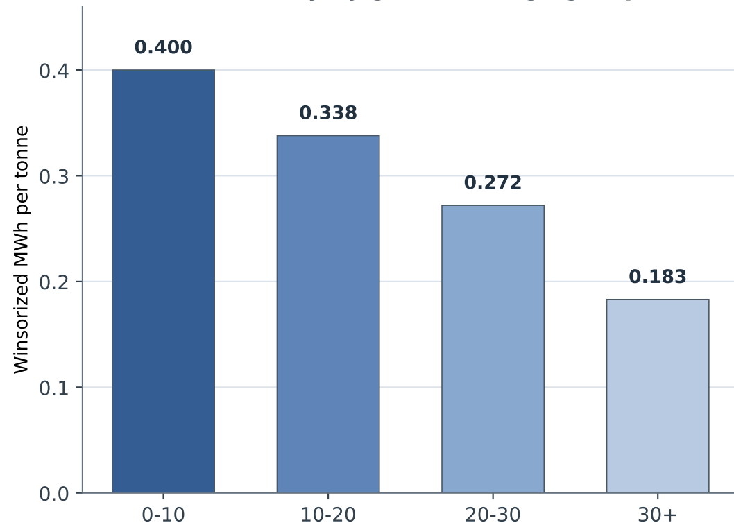
A. Mean efficiency by generator age group
