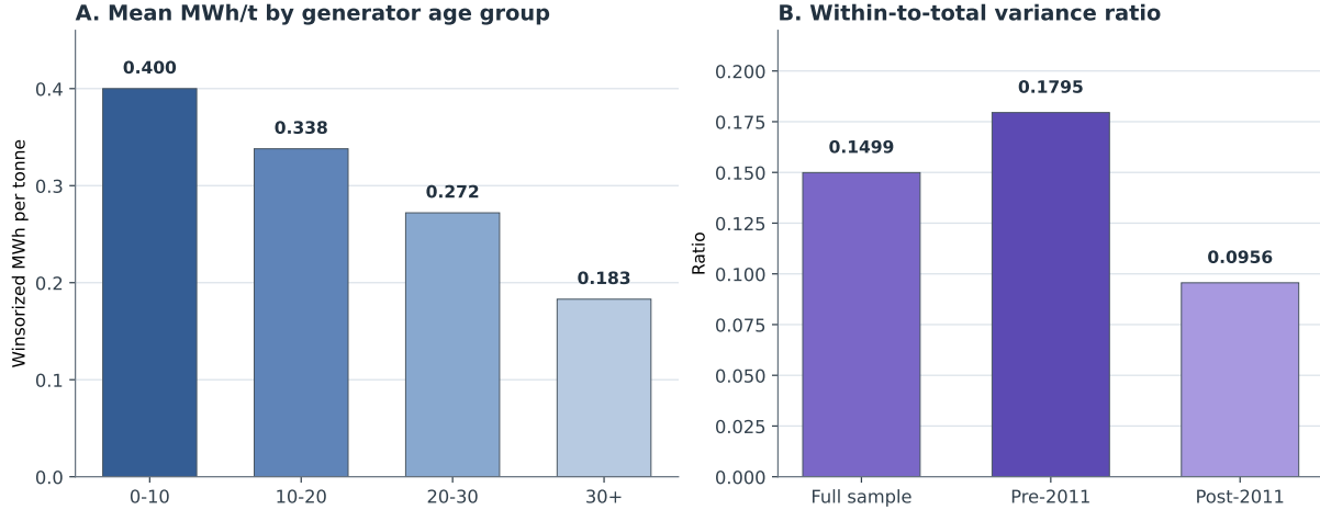
Figure 3: Mean electricity recovery intensity declines across generator age groups, while the within-to-total variance ratio stays low in the full sample and in pre/post-Fukushima splits.
