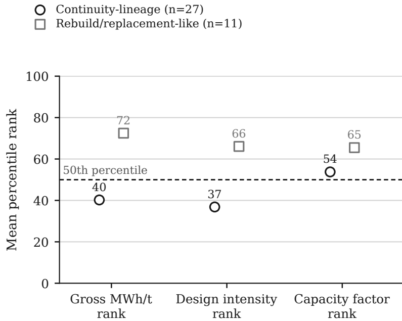
Figure A.1: Mean within-fiscal-year percentile ranks in the first complete year after reported entry for continuity-lineage entrants ( n = 27 ) and rebuild/replacement-like entrants ( n = 11 ). Metrics are gross MWh/t, generator design intensity (installed kW per t/day of processing capacity), and annual electrical capacity factor among engineering-valid generator-years; the dashed line marks the 50th percentile. The forward-dated/placeholder category ( n = 6 ) is omitted because support is sparse. All contrasts are descriptive.
