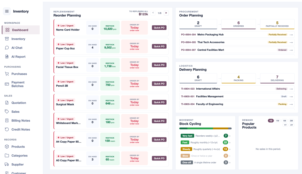
Figure 4.1 Dashboard page
