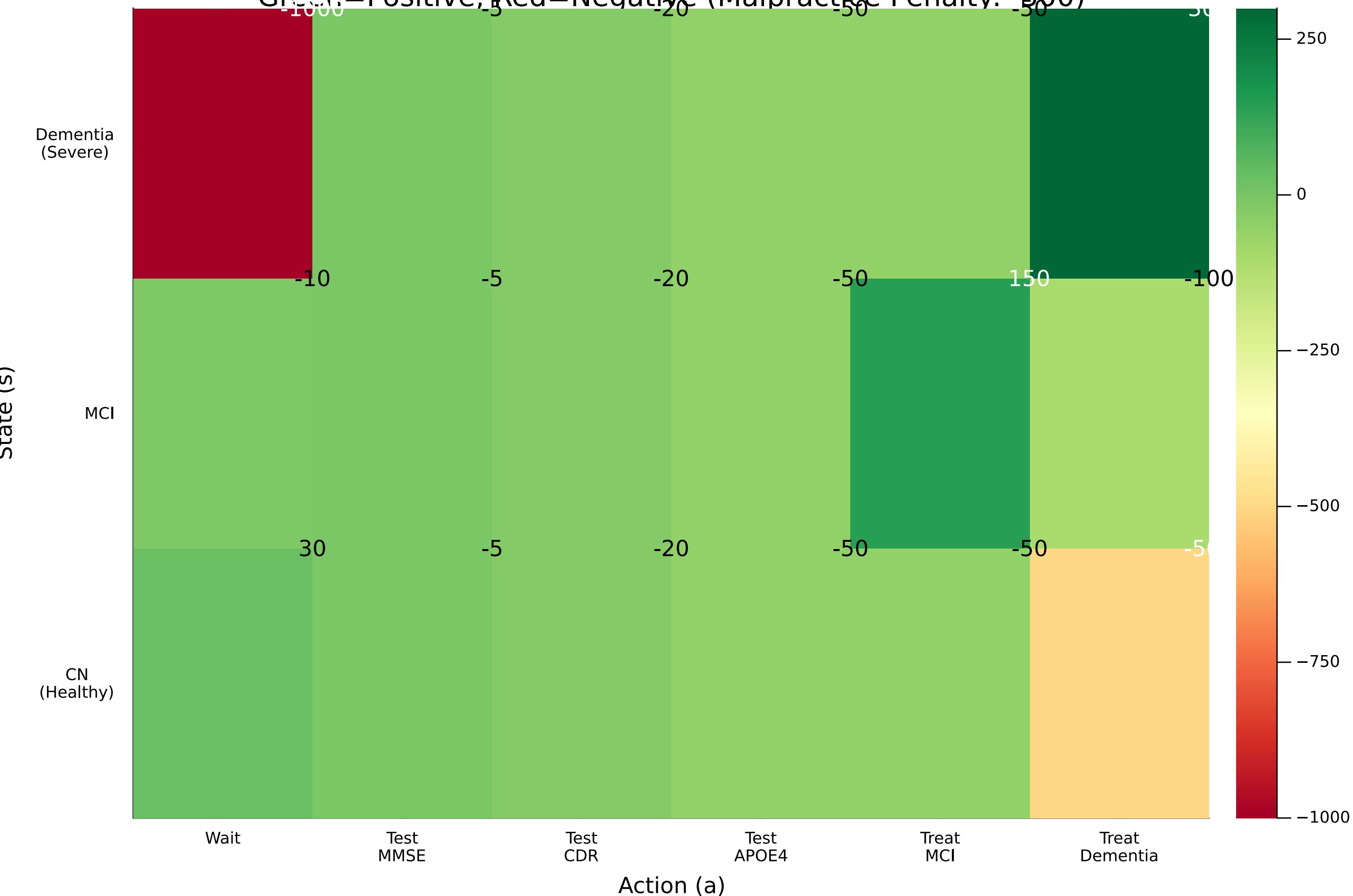
Reward Function R(s, a) Green=Positive, Red=Negative (Malpractice Penalty: -500)
