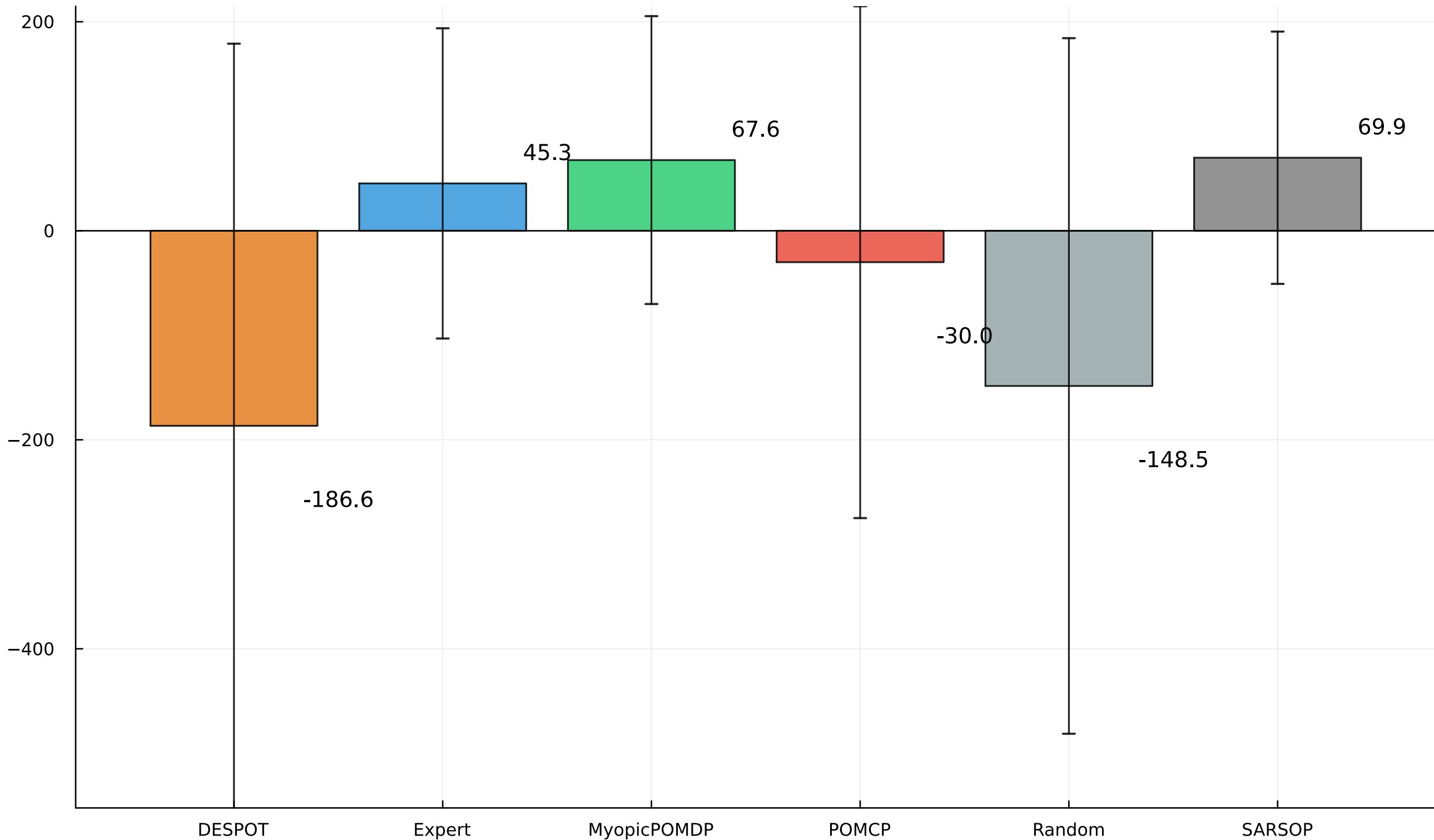
Average Reward Comparison Across Policies (N=1,000 Patients)
