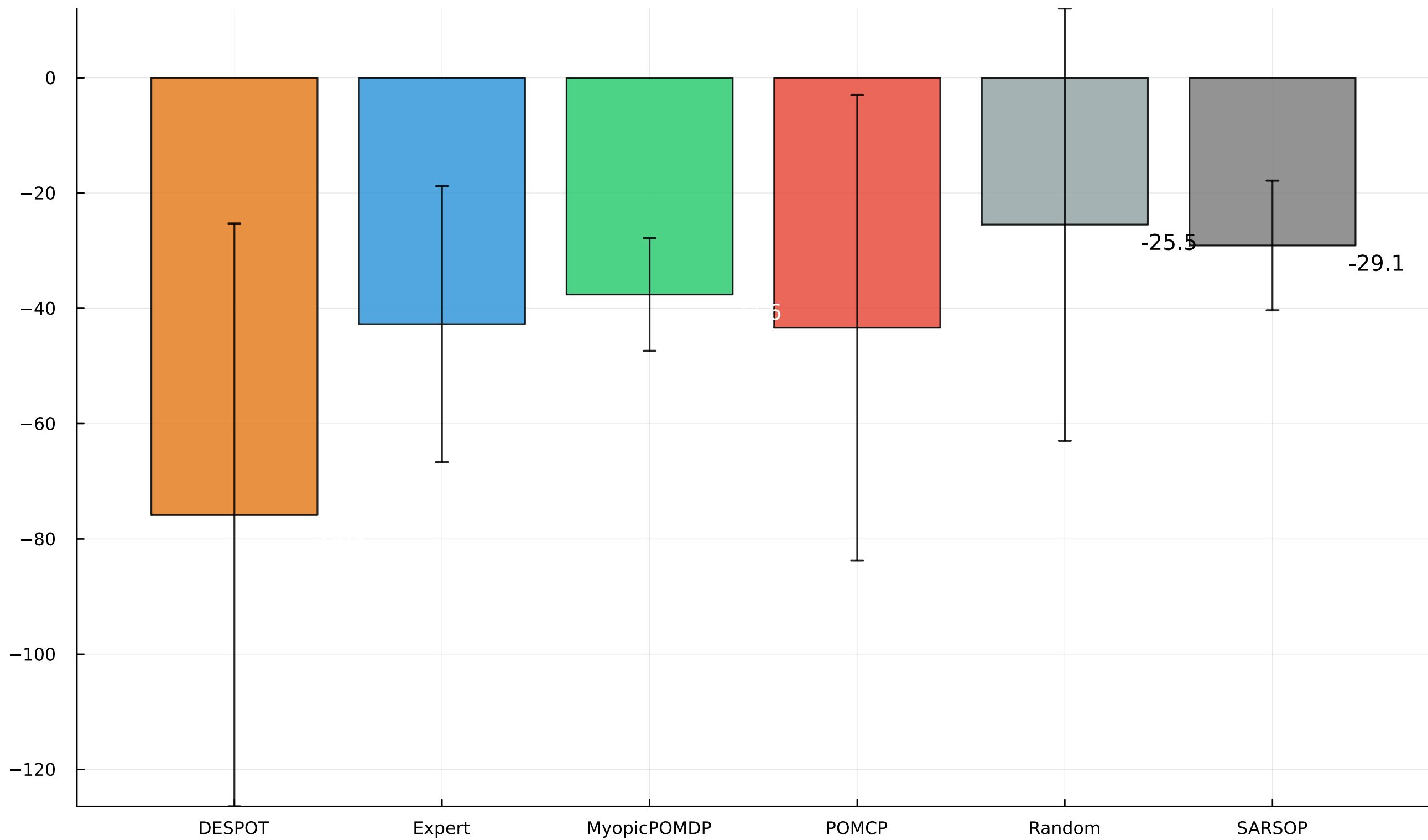
Average Testing Cost per Policy
