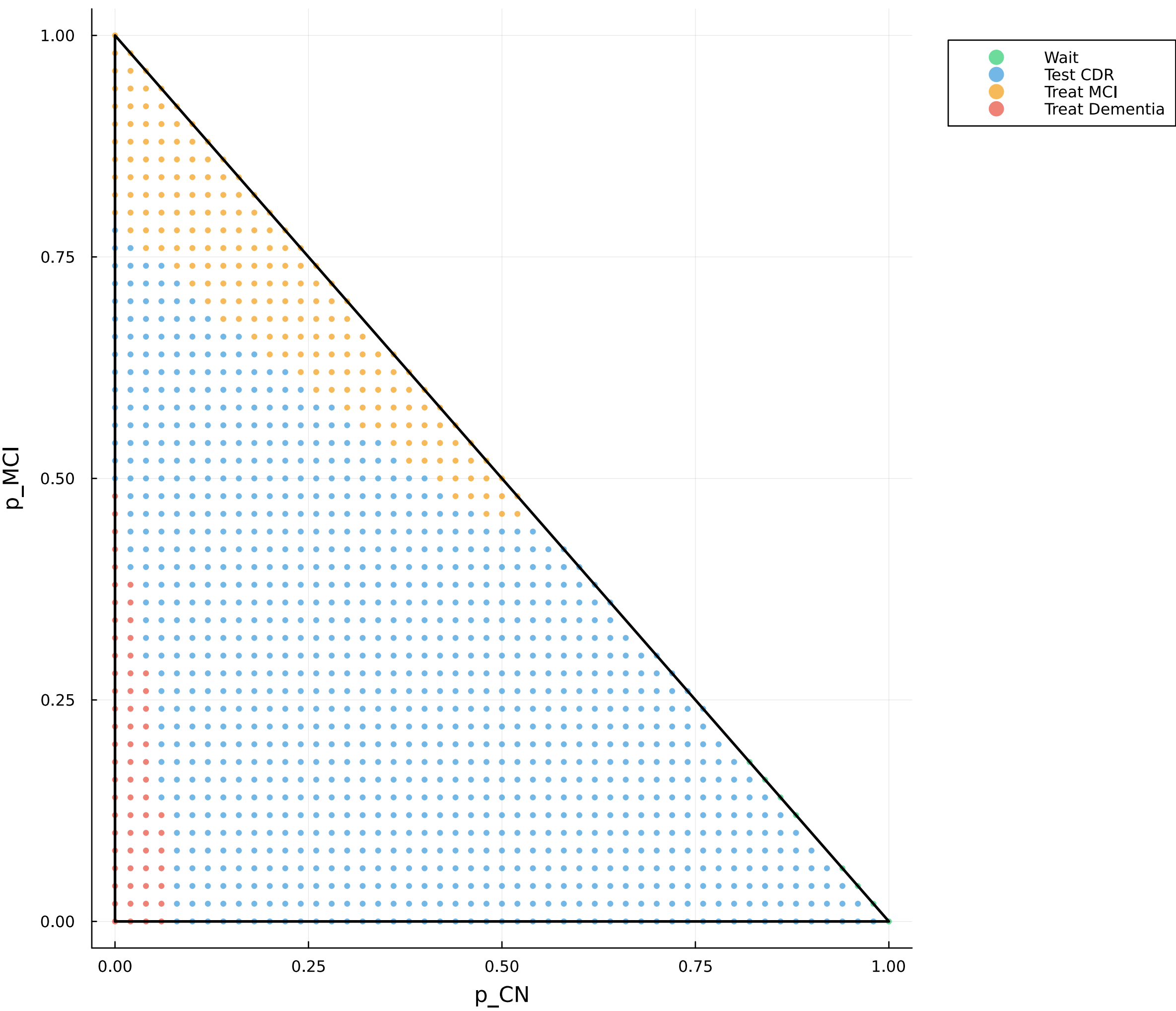
SARSOP Decision Regions over Belief Simplex
