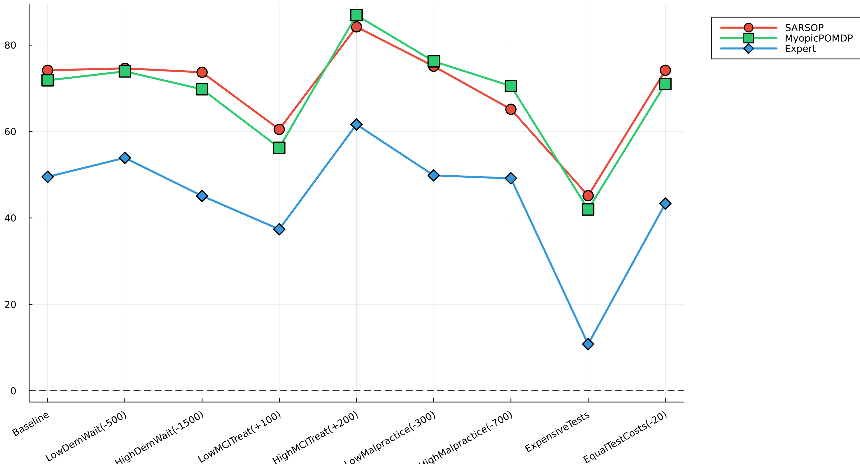
Sensitivity of Average Reward to Reward Function Variations
