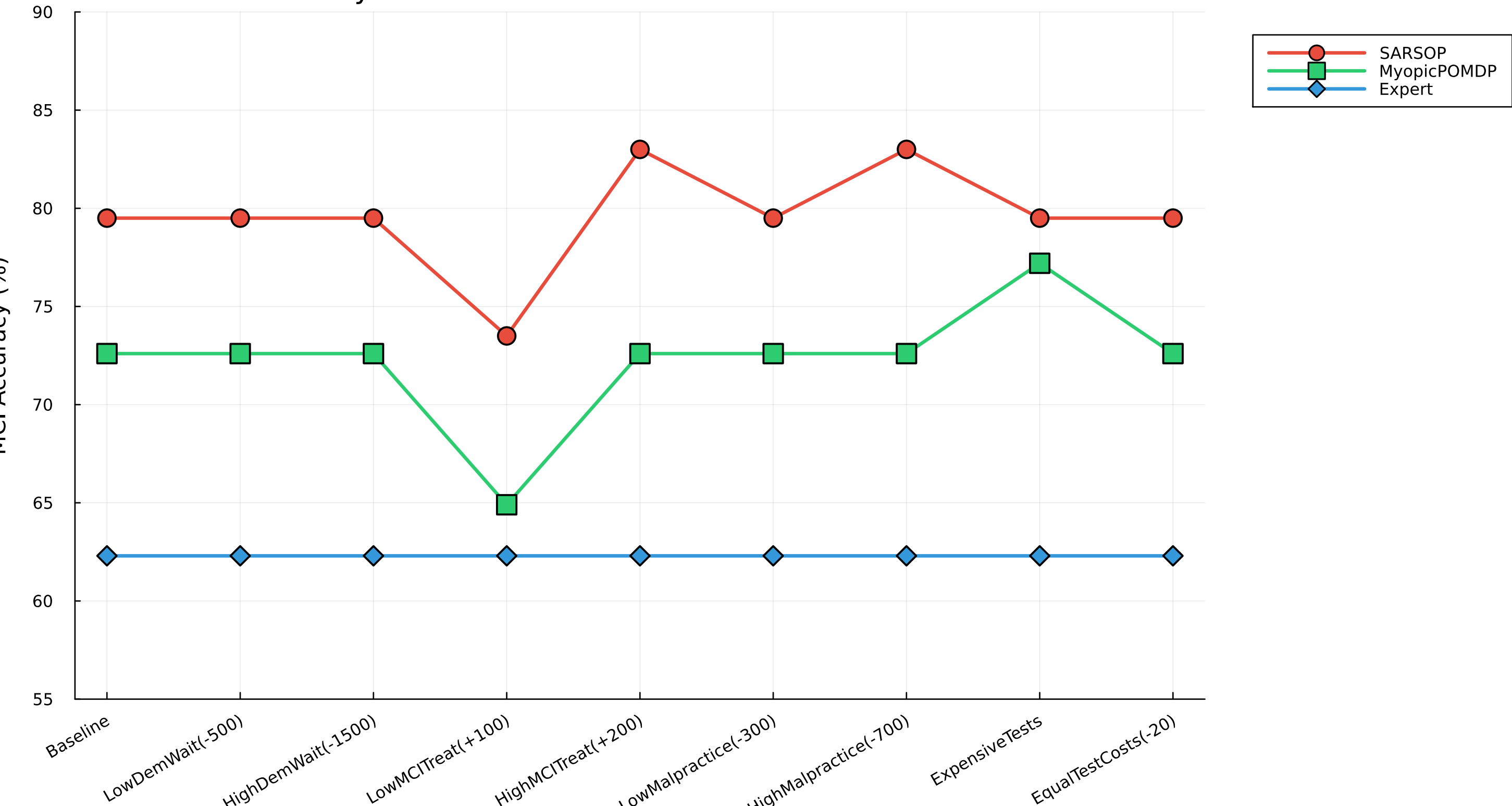
Sensitivity of MCI Detection to Reward Function Variations
