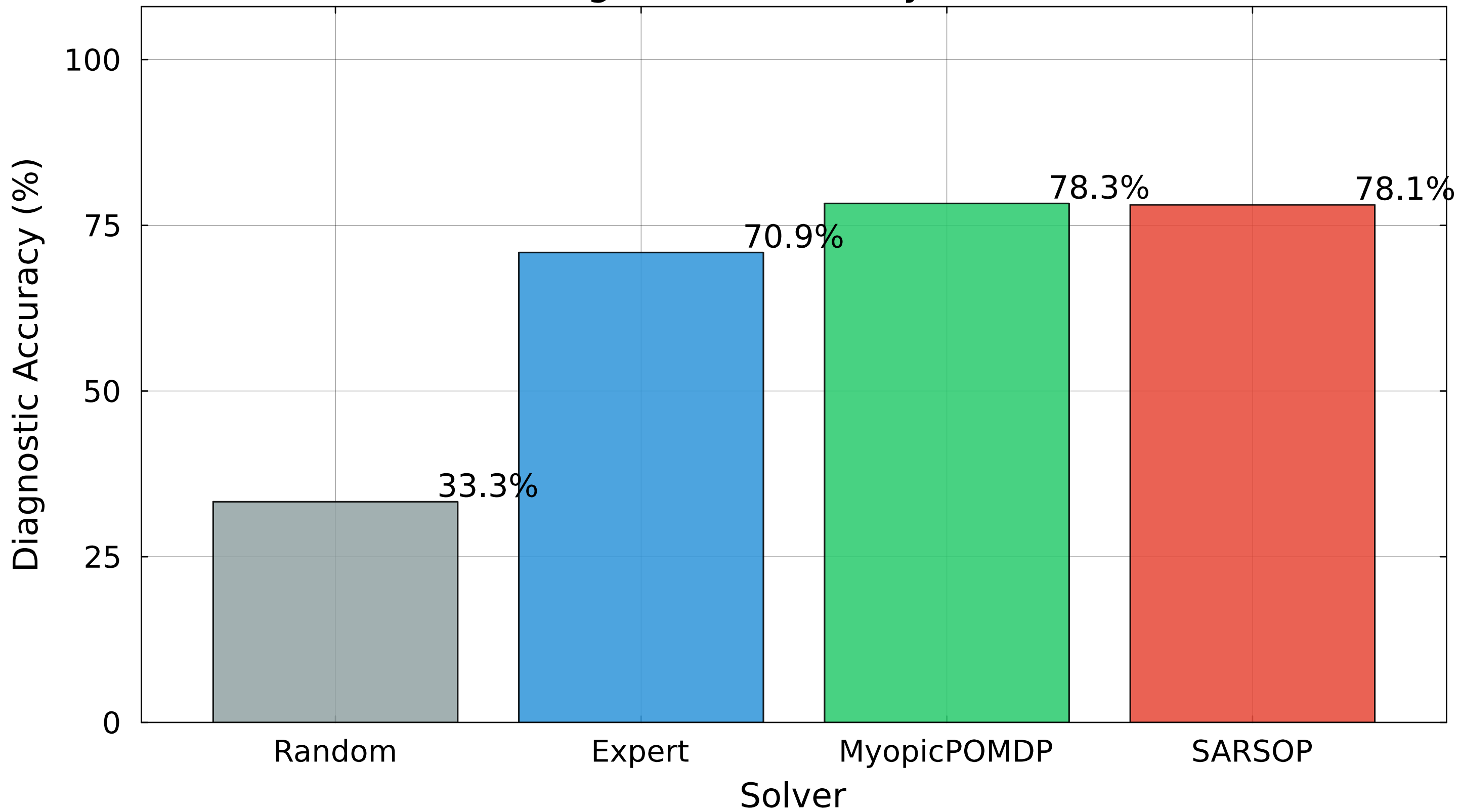
Overall Diagnostic Accuracy (N = 100000)
