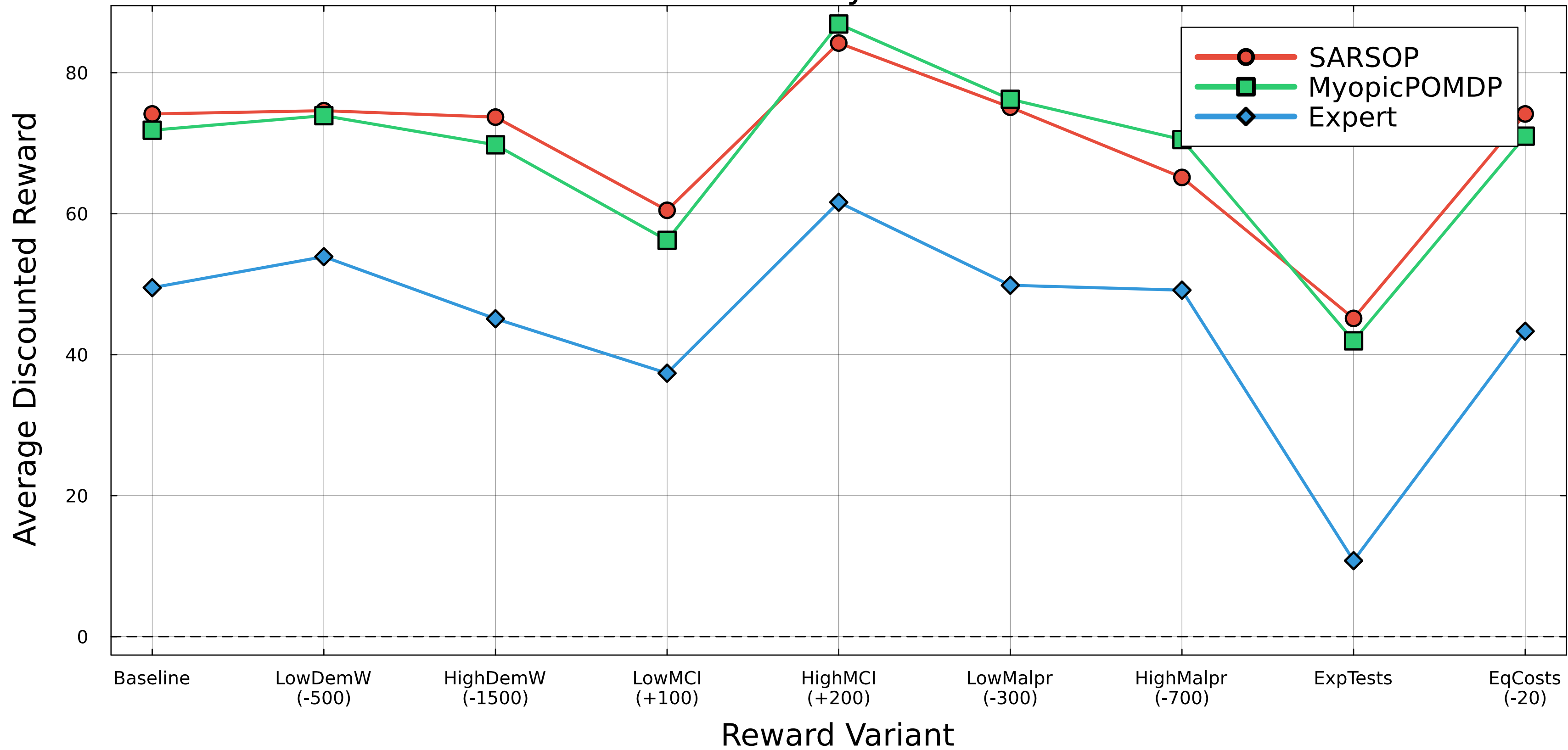
SARSOP Reward Sensitivity Across Reward Variants
