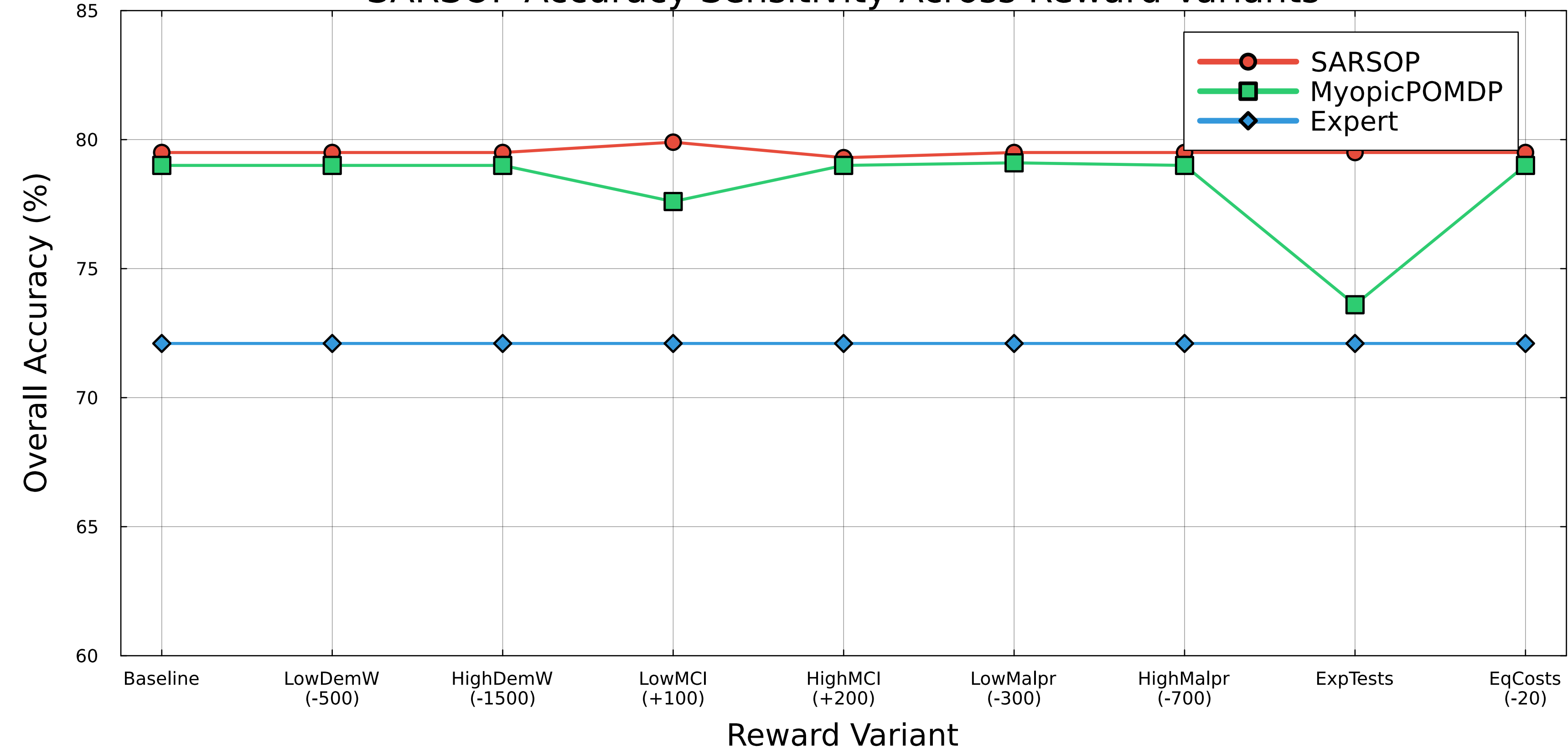
SARSOP Accuracy Sensitivity Across Reward Variants
