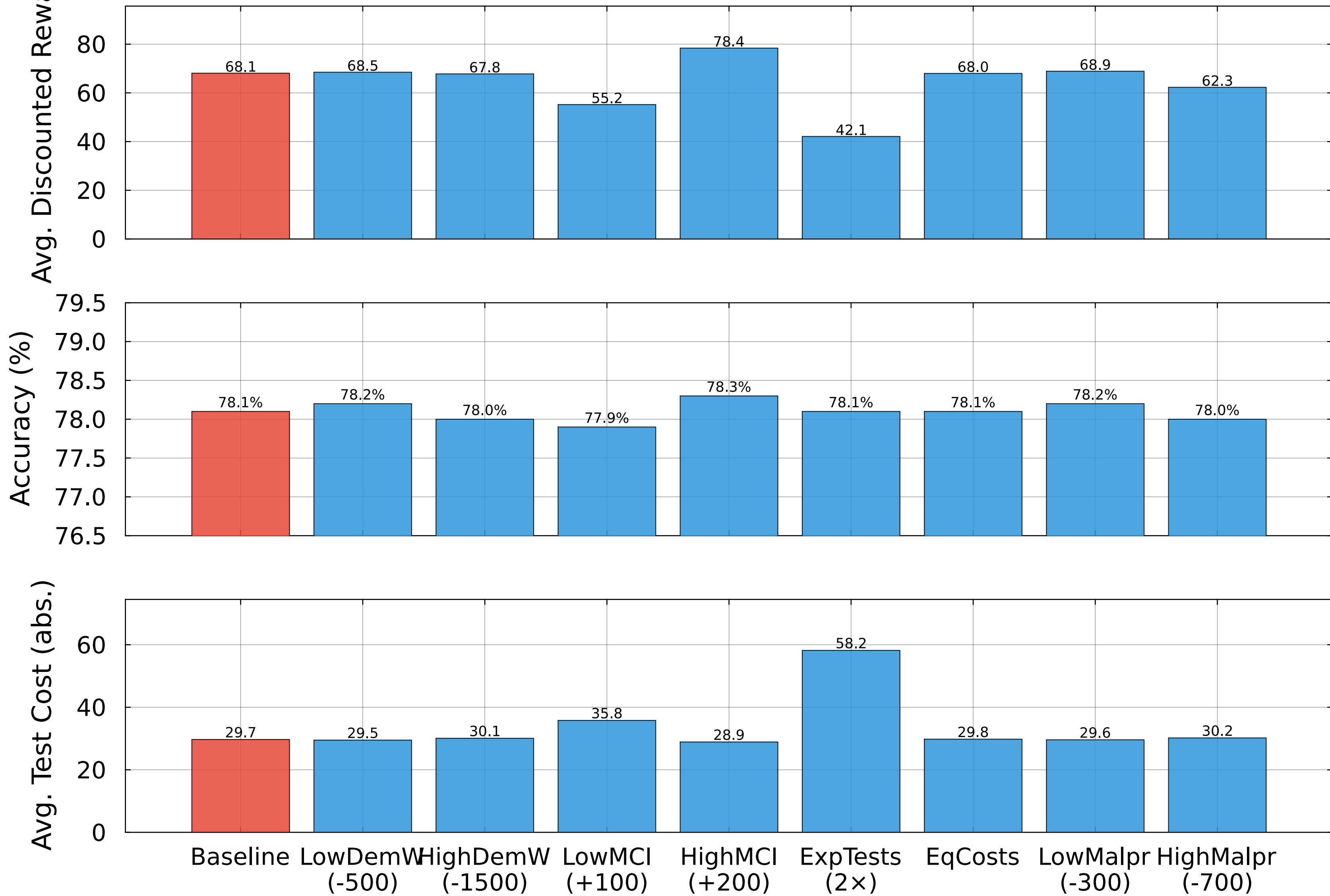
SARSOP Sensitivity Across Reward Variants
