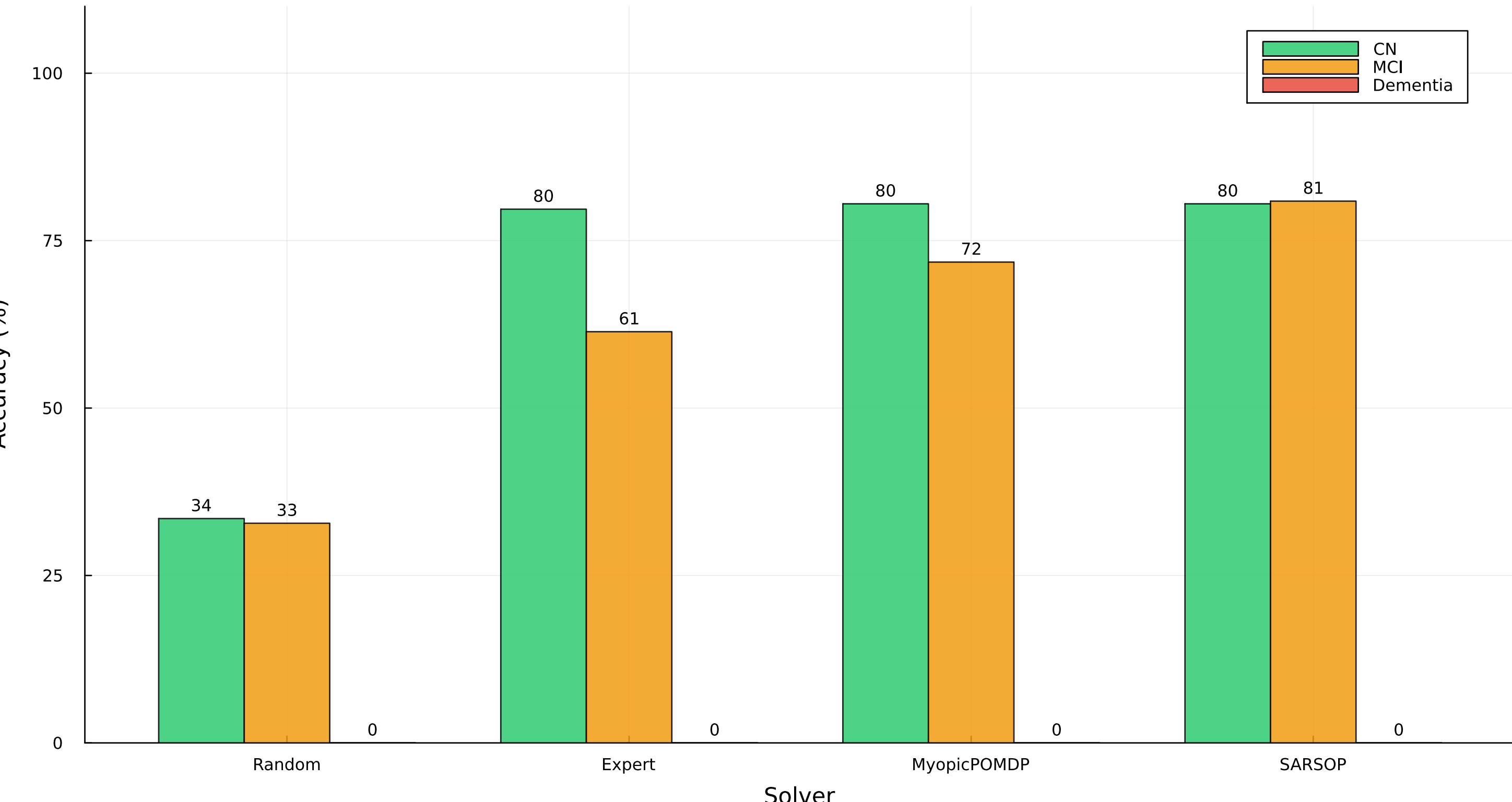
Per-State Diagnostic Accuracy (N=100000)
