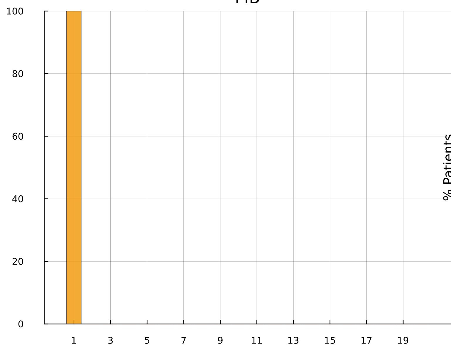
FIB
