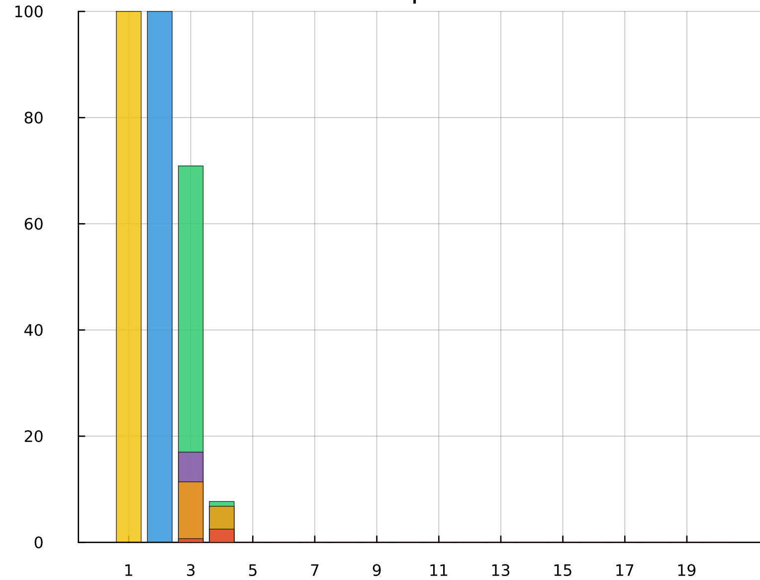
Random
