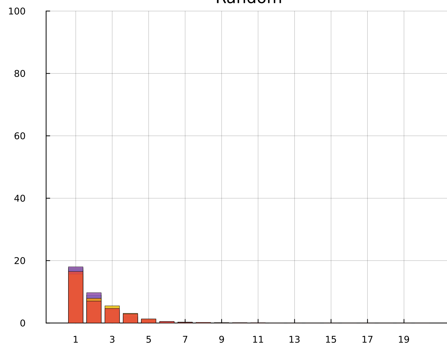
Random
