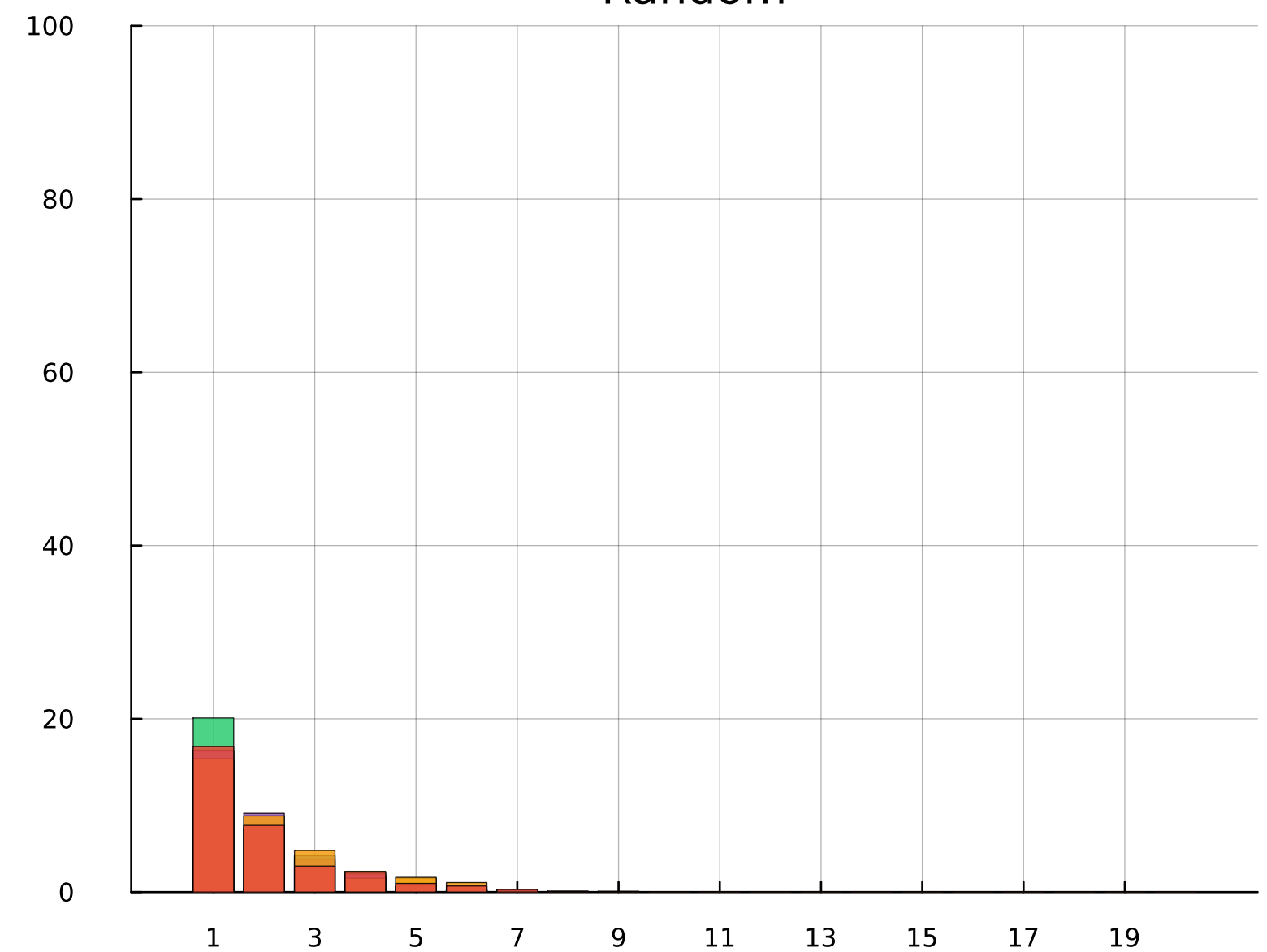
Random
