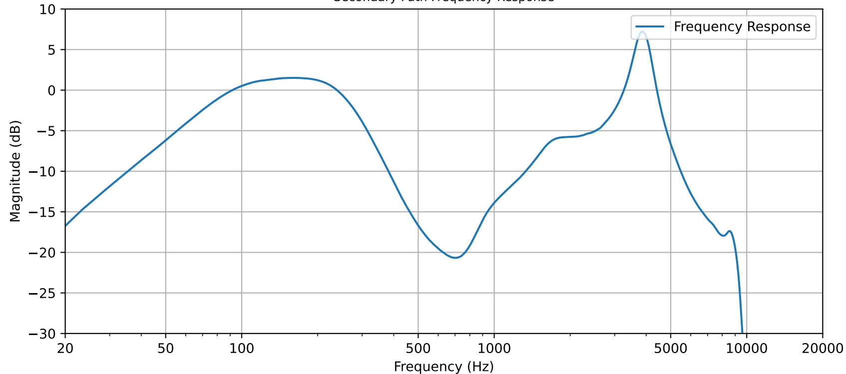
Secondary Path Frequency Response
