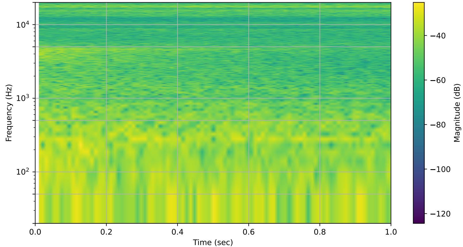
Error Spectrogram
