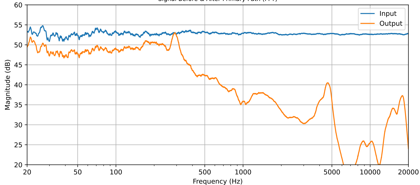
Signal Before & After Primary Path (FFT)
