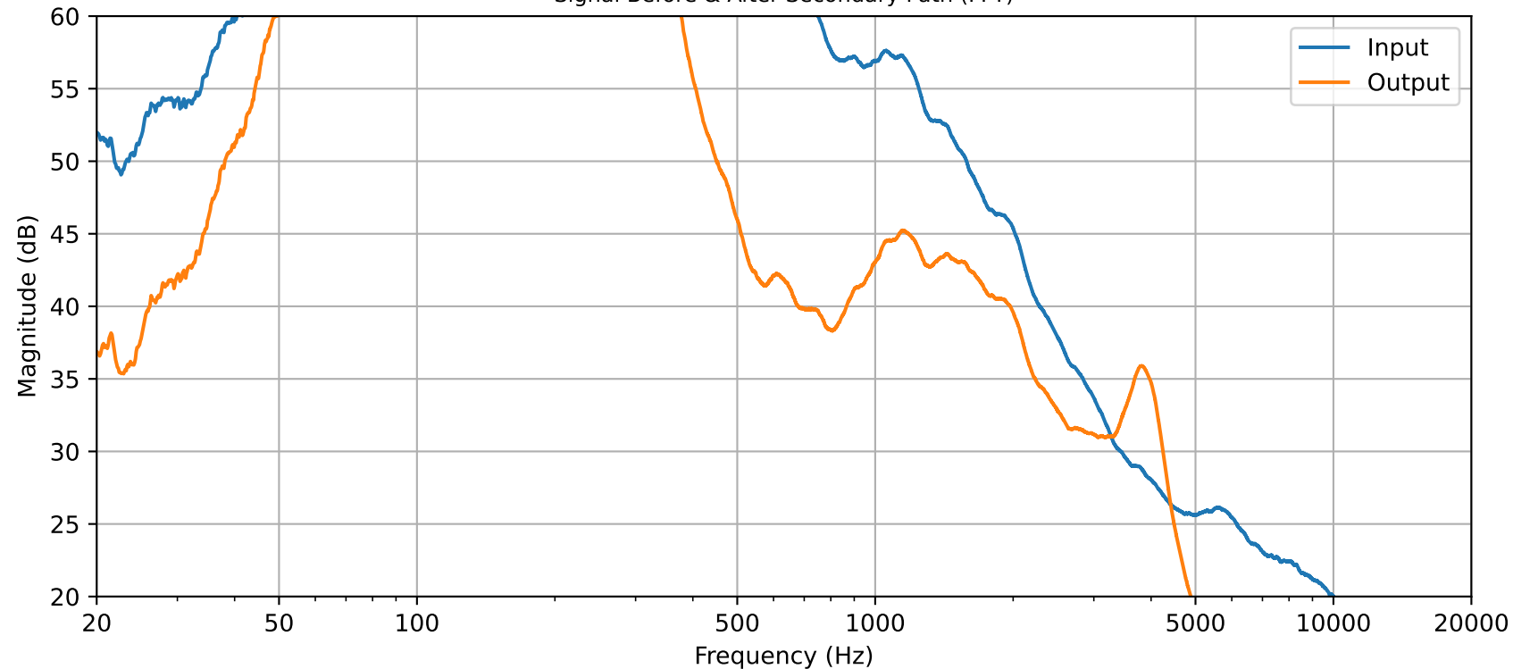
Signal Before & After Secondary Path (FFT)
