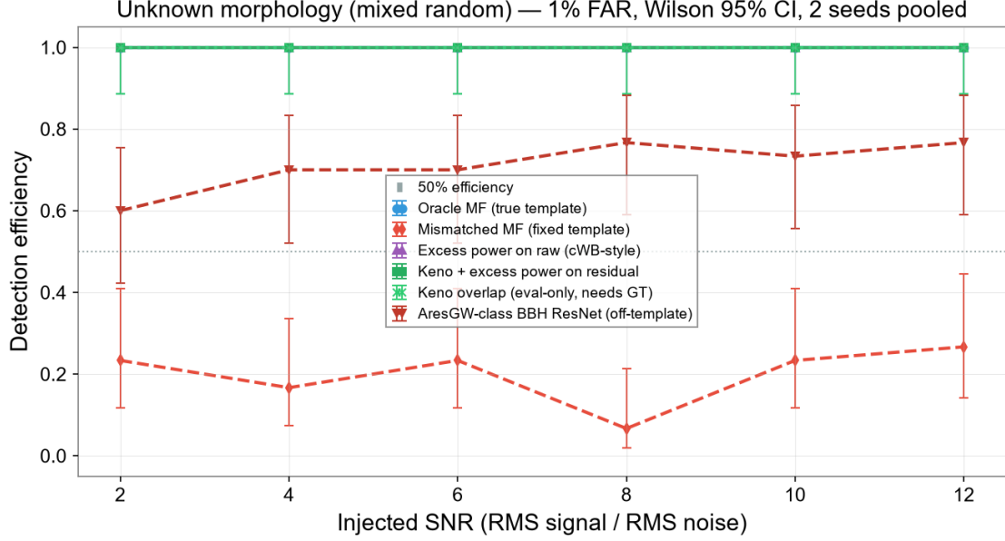
Figure 2: Detection efficiency versus injected SNR at 1% FAR for unknown morphologies. Baselines include raw excess power, mismatched matched filtering, and a BBH-trained ResNet control.
