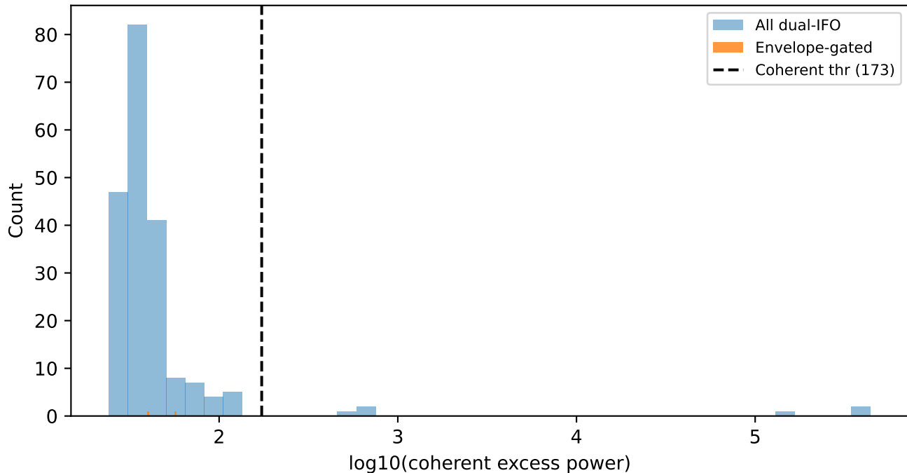
Dual-IFO noise coherent EP (gated vs ungated)
