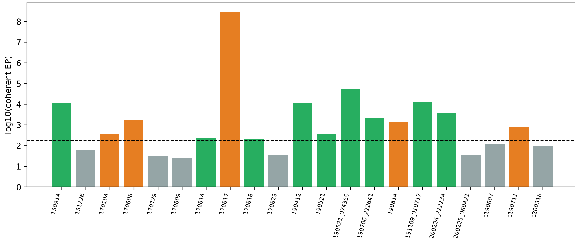
GWTC/cWB follow-up (green=YES, orange=envelope veto, gray=miss)
