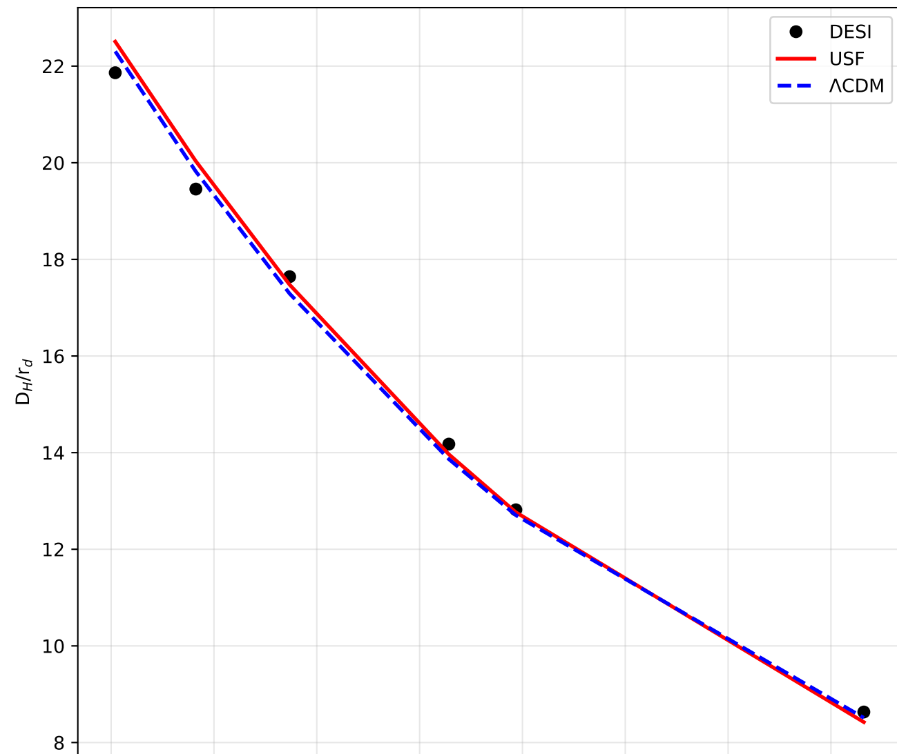
Hubble distance
