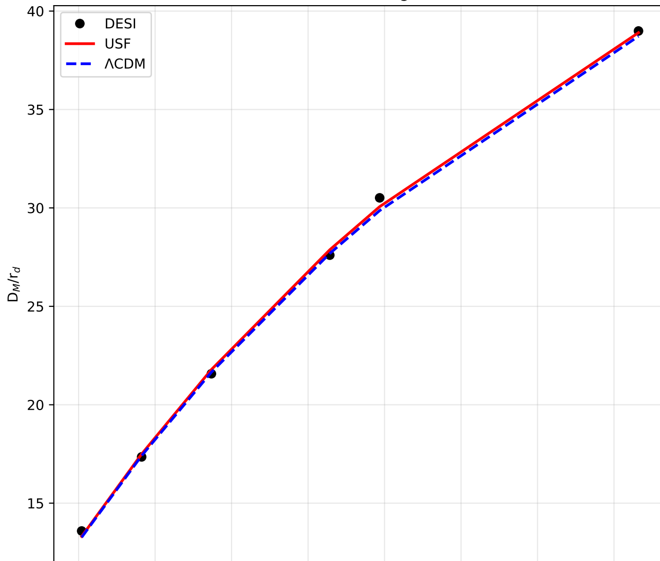
Transverse comoving distance
