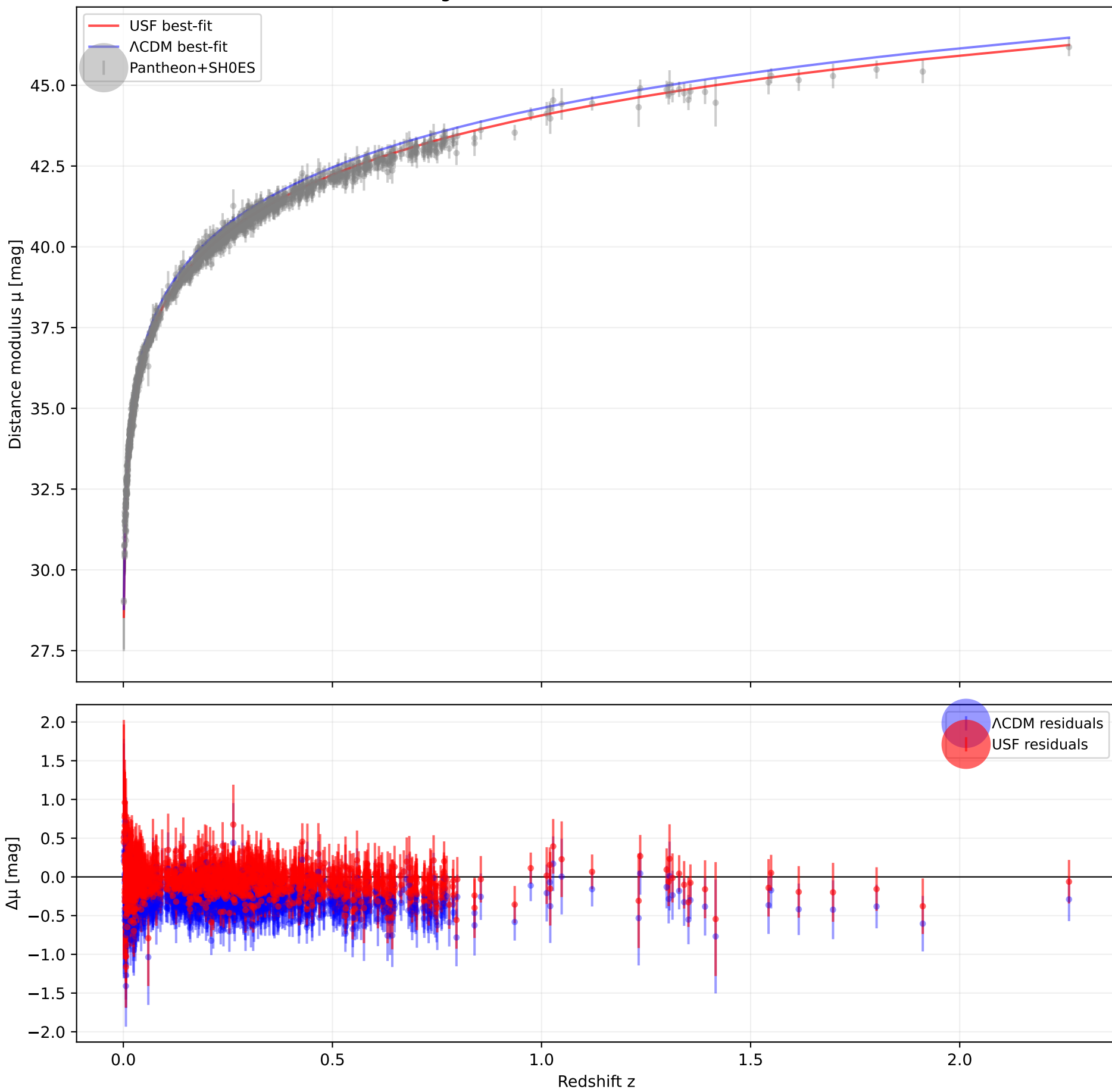
Hubble diagram - USF and \Lambda CDM vs Pantheon+SH0ES
