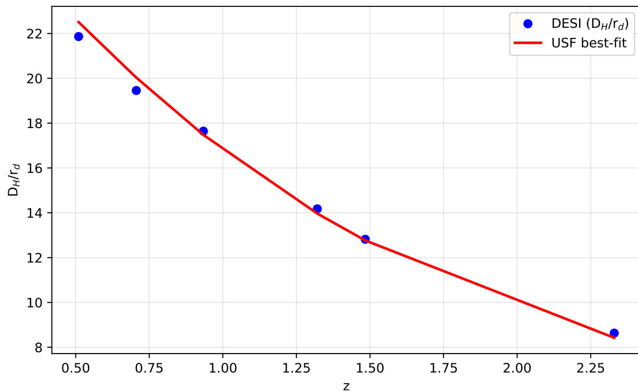
Hubble distance
