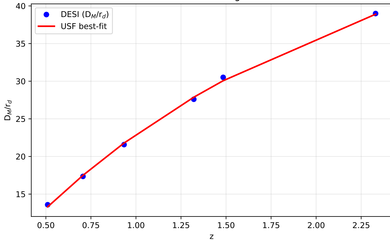
Transverse comoving distance
