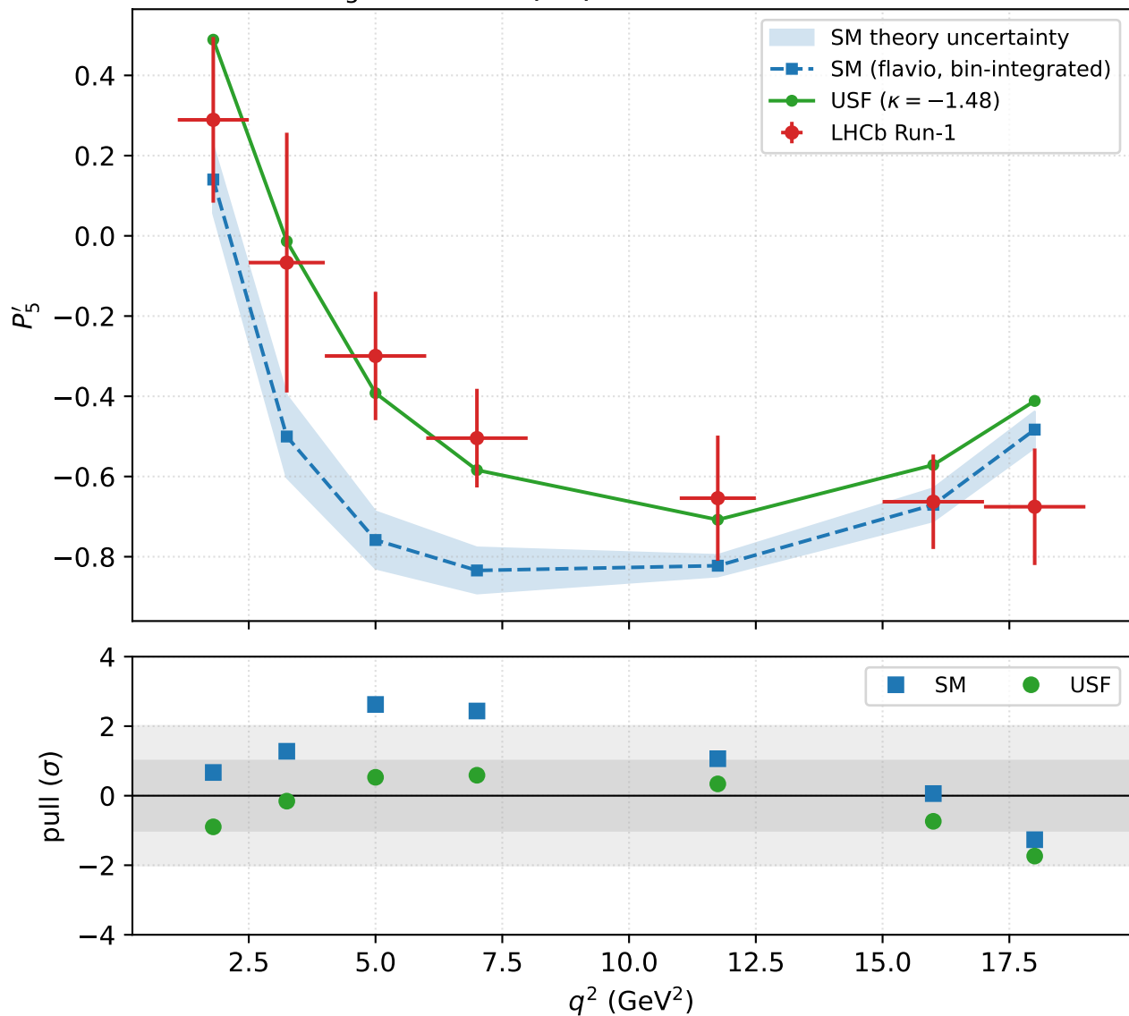
P'_5 in B^0 \rightarrow K^{*0} \mu^+ \mu^- : data, SM and USF
