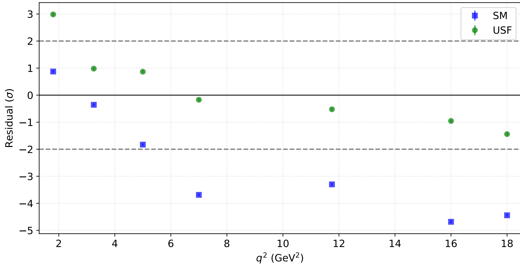
Normalised residuals: SM vs. USF
