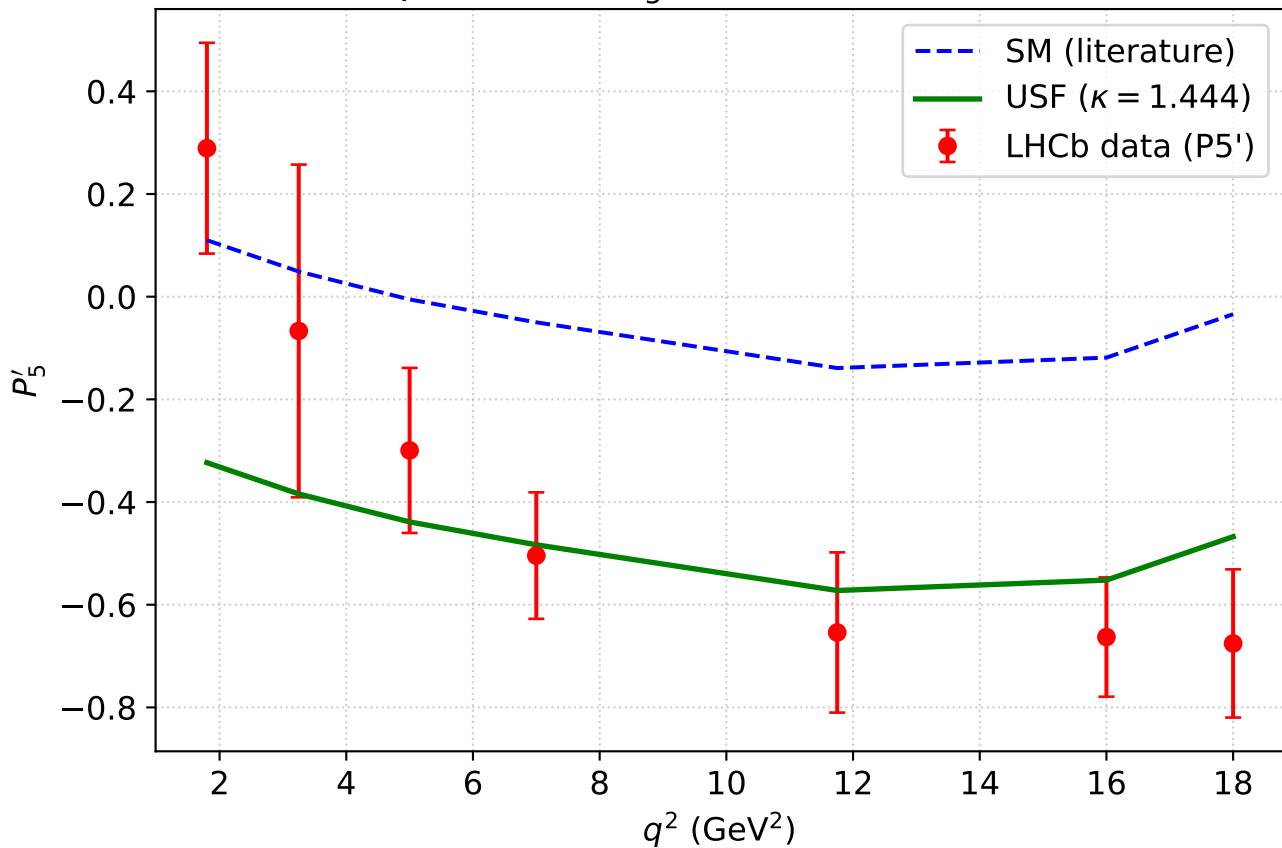
Spectrum of P'_5 : data vs. SM vs. USF
