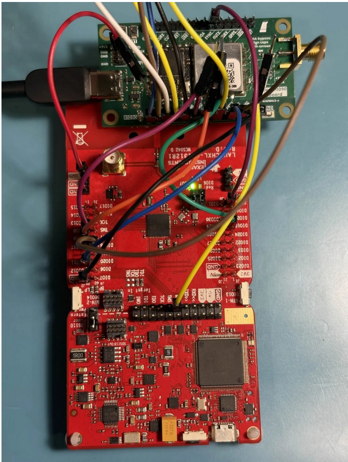
ADSBee m1090 Eval Board attached to a CC1312R1 Launchpad. Note that jumpers to the built-in debugger have been removed, and the launchpad is being powered by 3.3V stolen from the SWD header on the CC1312. Power can optionally be supplied via the Launchpad's built-in Micro USB connector instead.
